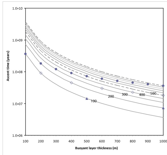
Figure 2. Ascent time as a function of buoyant layer thickness for gypsum. Each line represents a constant overburden thickness from 100–1000 m, with the 500 and 1000 m lines dashed. The points represent particular buoyant layer to overburden thickness ratios. Triangles are 5:1, diamonds 2:1 and filled circles 1:1.
