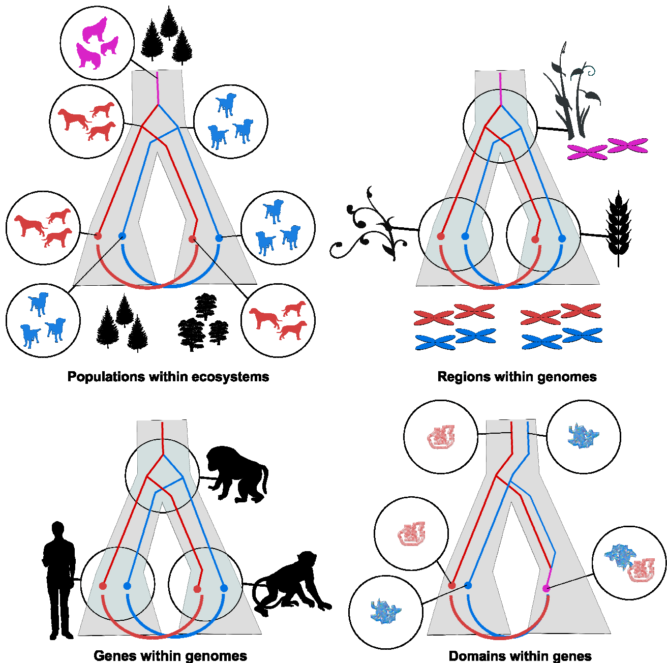
Figure 1. Nested Evolutionary Histories: Containing (e.g. species) trees (grey area) with nested (e.g. gene) trees (red/blue) inside. Semicircles denote orthologous or orthology-like relations. On the top level (top left panel), subpopulations unique to a particular ecological niche are nested within populations, and within subpopulations in turn, the histories of individual genealogies are nested. In this sense, niche segregation within a site is a form of duplication event, whereas migration to novel habitats correspond to speciation events at this level. In addition, genes lie within genomes that are subject to whole-genome or chromosome-scale duplication events (top right panel, bottom left panel), which strongly influences genome evolution and involve discordances between the histories of components and wholes, and protein domains within genes may reshuffle over evolutionary time
