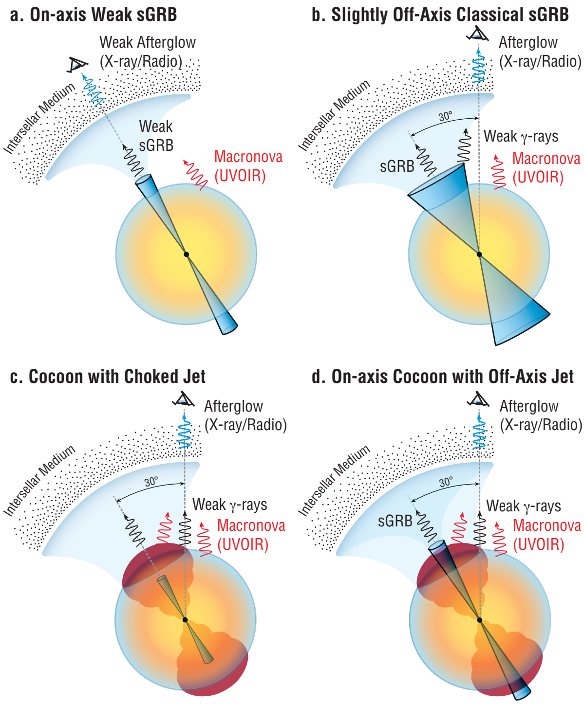
Figure 5: Model schematics considered in this paper. In each panel, the eye indicates the line of sight to the observer. (A) A classical, on-axis, ultra-relativistic, weak short gamma-ray burst (sGRB). (B) A classical, slightly off-axis, ultra-relativistic, strong sGRB. (C) A wide-angle, mildly-relativistic, strong cocoon with a choked jet. (D) A wide-angle, mildly-relativistic, weak cocoon with a successful off-axis jet.
