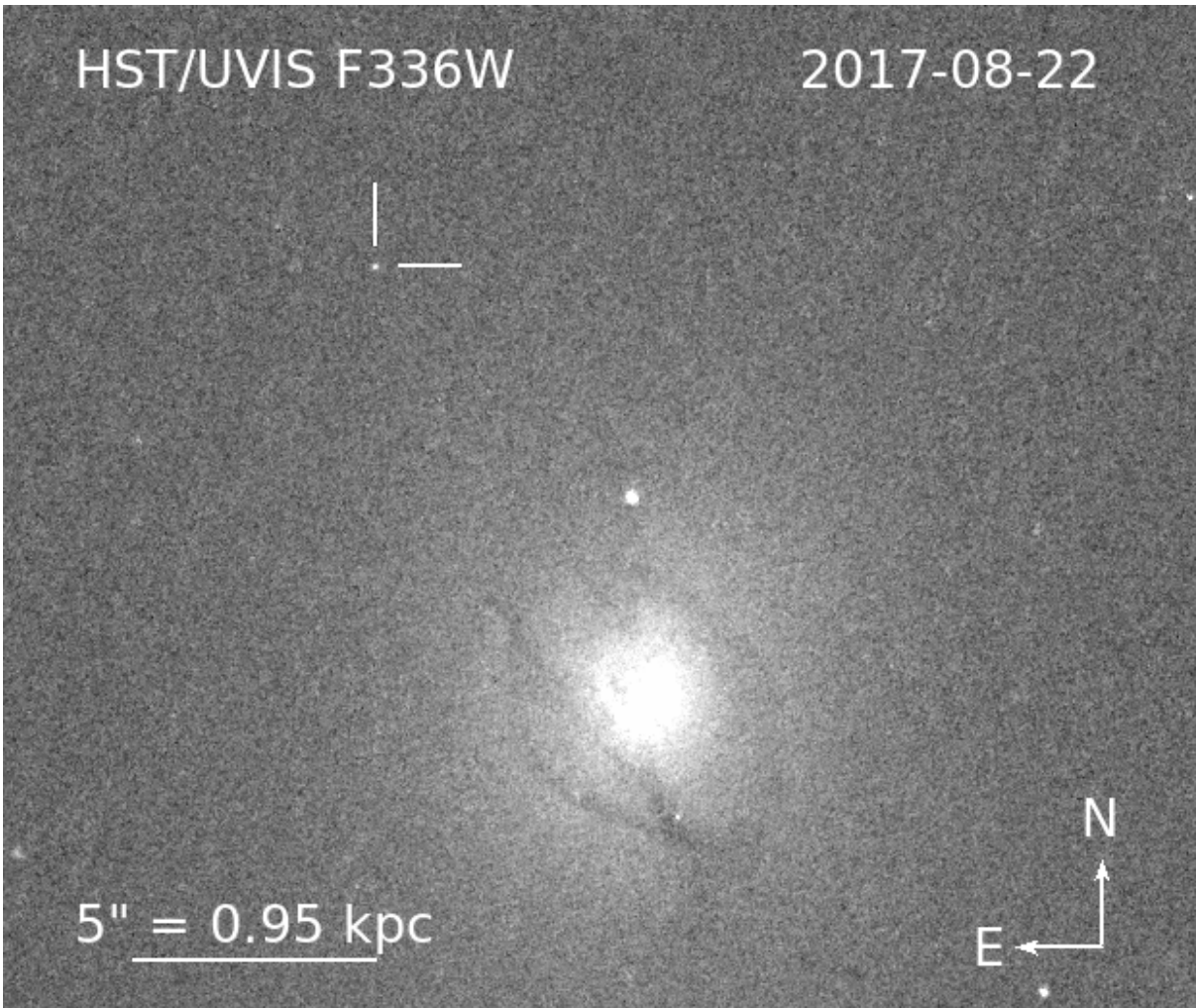
Figure S1: Hubble Space Telescope WFC3/F336W ultraviolet image of EM170817 and NGC 4993, taken 2017 August 22. North is up, east is the to left, and a 5" scale-bar is indicated. The position of the transient is shown with tick marks. Dust lanes are visible toward the center of NGC 4993.
