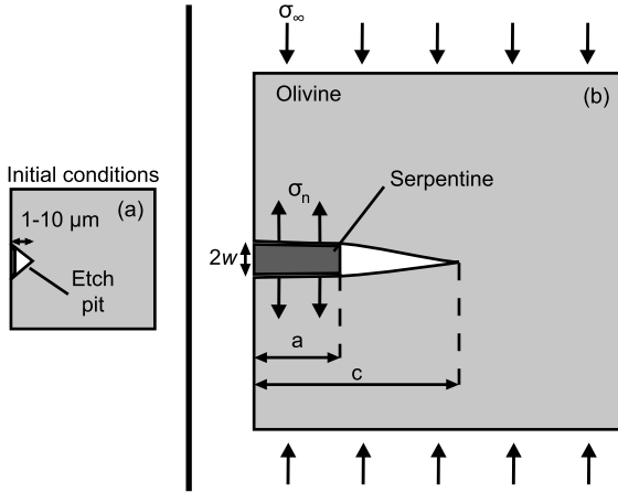
Fig. 3. Geometry of crack propagation model. (a) Initial conditions. The pre-existing fracture is assumed to be an etch pit formed by anisotropic olivine dissolution. (b) Geometry for crack propagation as serpentine precipitates into the crack. a and w are the length and half-width of the serpentine mineral. c is the crack length.
