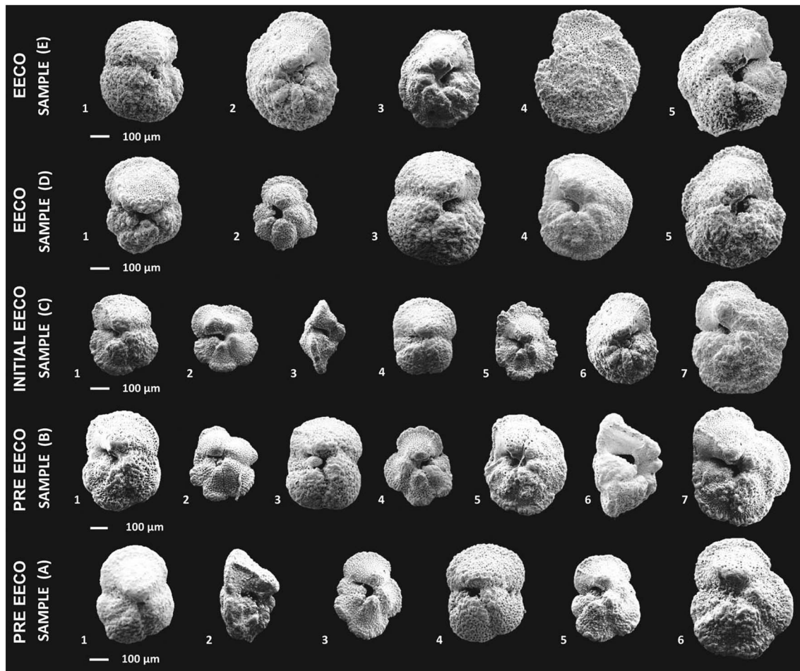
Figure 5. SEM images showing variations in size of representative Morozovella species from the >300 μm fraction for the five analyzed “bleaching” samples at Site 1051. Sample A (443.58 mbsf) 1–2: M. subbotinae , 3: M. gracilis ; 4: M. aequa ; 5: M. marginodentata ; 6: M. crater . Sample B (433.50 mbsf) 1: M. subbotinae ; 2: M. gracilis ; 3: M. aequa ; 4: M. marginodentata ; 5: M. aragonensis ; 6–7: M. crater . Sample C (425.40 mbsf) 1: M. subbotinae ; 2–3: M. gracilis ; 4: M. aequa ; 5: M. marginodentata ; 6: M. aragonensis ; 7: M. crater . Sample D (411.80 mbsf) 1: M. subbotinae ; 2: M. gracilis ; 3: M. aequa ; 4: M. aragonensis ; 5: M. crater . Sample E (395.65 mbsf) 1: M. aequa ; 2–3: M. aragonensis ; 4–5: M. crater . Note that almost the whole Morozovella population displays a transitory reduction in size at sample C (initial EECO).
