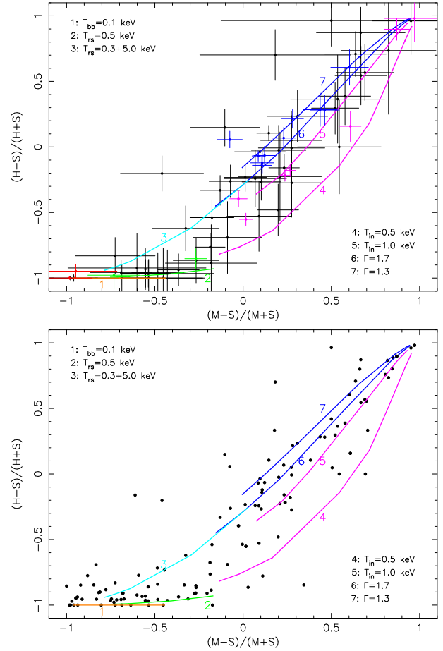
Fig. 14. Top panel: color-color diagram for sources brighter than \approx 10^{37} erg s ^{-1} , with respective error bars. Bottom panel: color-color diagram for the all sources in the S3 chip, without error bars. In addition to the models shown in Fig. 12, we have also overplotted a two-temperature thermal plasma model ( kT_{rs,1} = 0.3 keV, kT_{rs,2} = 5.0 keV), normalised so that the high-temperature component accounts for 25% of the emitted flux.
