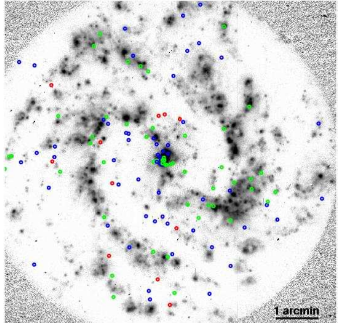
Fig. 17. Location of the discrete X-ray sources classified according to their color group (red for group A sources; green for group B; blue for group C), overplotted onto a continuum-subtracted H\alpha image of M 83. North is up, East is left. The H\alpha image was taken by Stuart Ryder from the Anglo-Australian Telescope.
