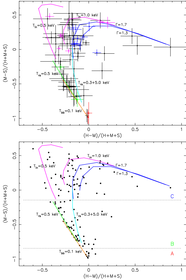
Fig. 15. Same as Fig. 14 for the alternative color indices. The three groups (A, B, C) are separated by the horizontal dotted lines.
