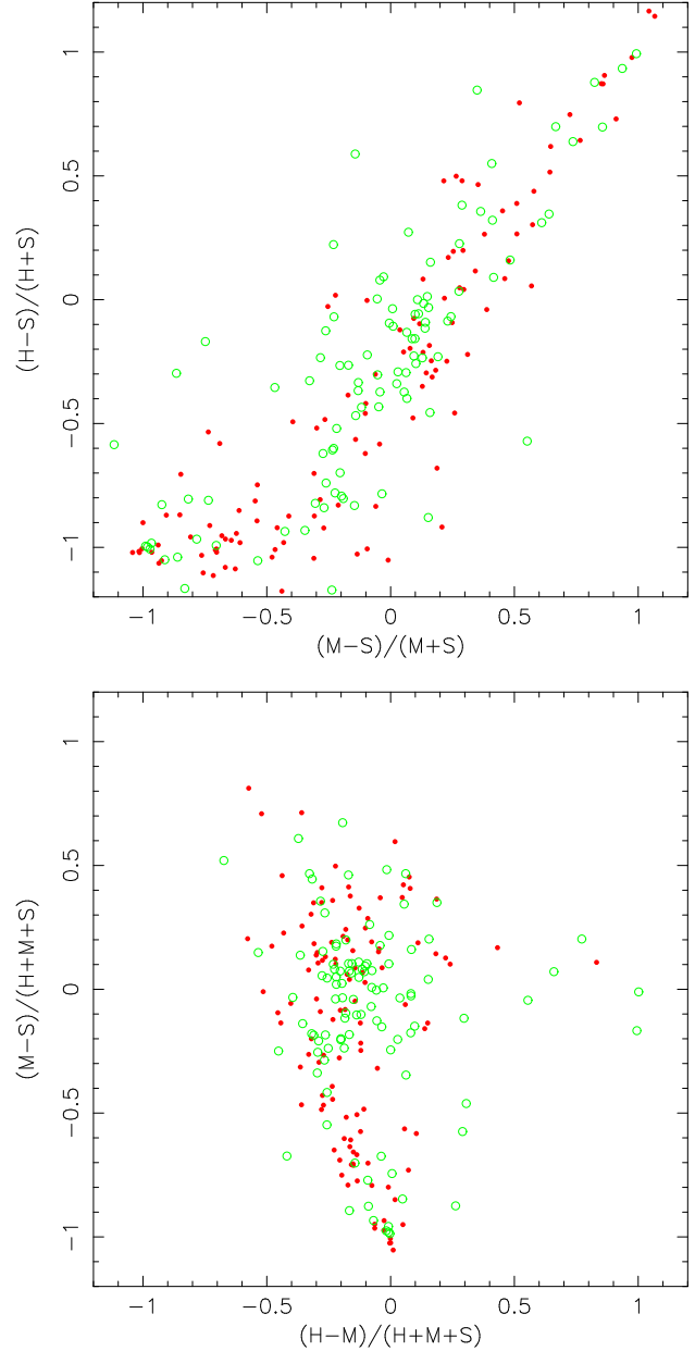
Fig. 21. Color-color plots for X-ray sources in M 83 and M 81, for conventional and alternative color indices (as defined in Sect. 5.2). Here the soft band is defined as 0.2–1.0 keV. Filled red circles represent M 83 sources, and open green circles represent M 81 sources. Error bars have been omitted.
