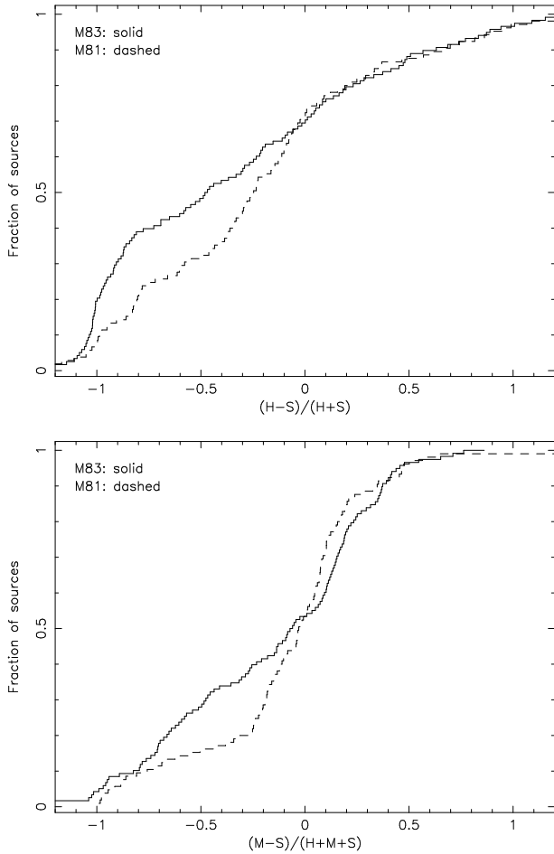
Fig. 22. The cumulative color distribution of the sources in M 83 (solid line) and M 81 (dashed line). S is defined here as the 0.2–1.0 keV band.
