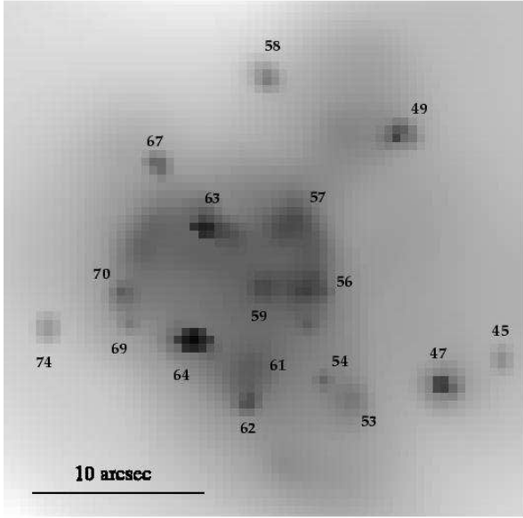
Fig. 2. Close-up view of the starburst nucleus. The source numbers refer to Table A.1. North is up, and East is left.
