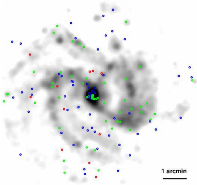
Fig. 20. Group A, B and C sources (green, red and blue circles respectively) overlotted on a map of the radio continuum emission at 6.3cm. The radio map is a combination of data from the VLA and Effelsberg radio telescopes, at a resolution of 12'' , and was produced by S. Sukumar, R. Allen, R. Beck & N. Neininger.
