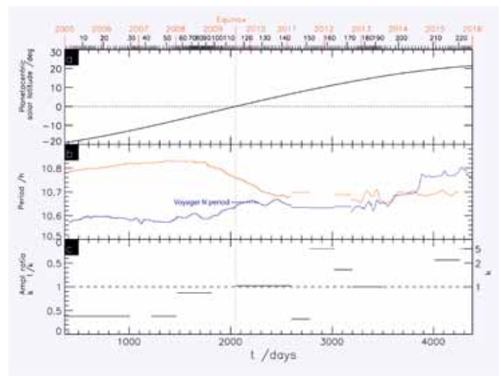
shows the northern (blue) and southern (red) PPO periods derived from Cassini MAG data. The blue dotted line shows the Voyager northern PPO period (see text). The bottom panel shows the north/south PPO amplitude ratio k , plotted directly for 0 < k < 1 (southern dominant), and as 1/k in the upper half for 1 < k < \infty (northern dominant). Dotted lines indicate lower limits on k for intervals when the southern PPO could not be discerned (indicating k > 5 ).
