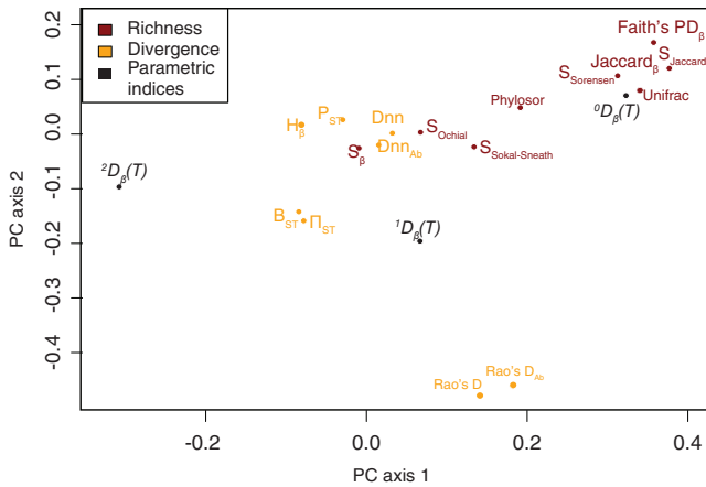
Fig. 3. Principal components analysis for Spearman's correlations between the \beta -diversity metrics shown in Table 1. Results represent measures taken from 800 simulated landscapes based on 100 simulated phylogenetic trees and eight landscape types defined in Table 2 (see online Appendix S2 for details). X and Y axes are scaled to reflect explained variance ( PC1 = 22.9\% ; PC2 = 15.6\% ). Where metrics are identified in Table 1 as mathematically identical, we include only one (e.g. Rao's D is plotted, but not Dpw). See Appendix S1 for equalities among indices.
