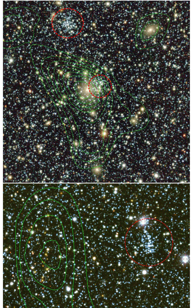
Figure 6. grz pseudo-colour images around star cluster positions with significant \lambda_{\text{MCMF}} measurements. The image shows the presence of galaxy clusters close to the star cluster positions. The top image shows the case with two star clusters next a galaxy cluster. The galaxy density contours (green) further highlight that the \lambda_{\text{MCMF}} peaks found are related to those galaxy clusters and not caused by stars leaking into the galaxy sample. Dashed red circles mark the locations of the star clusters.
