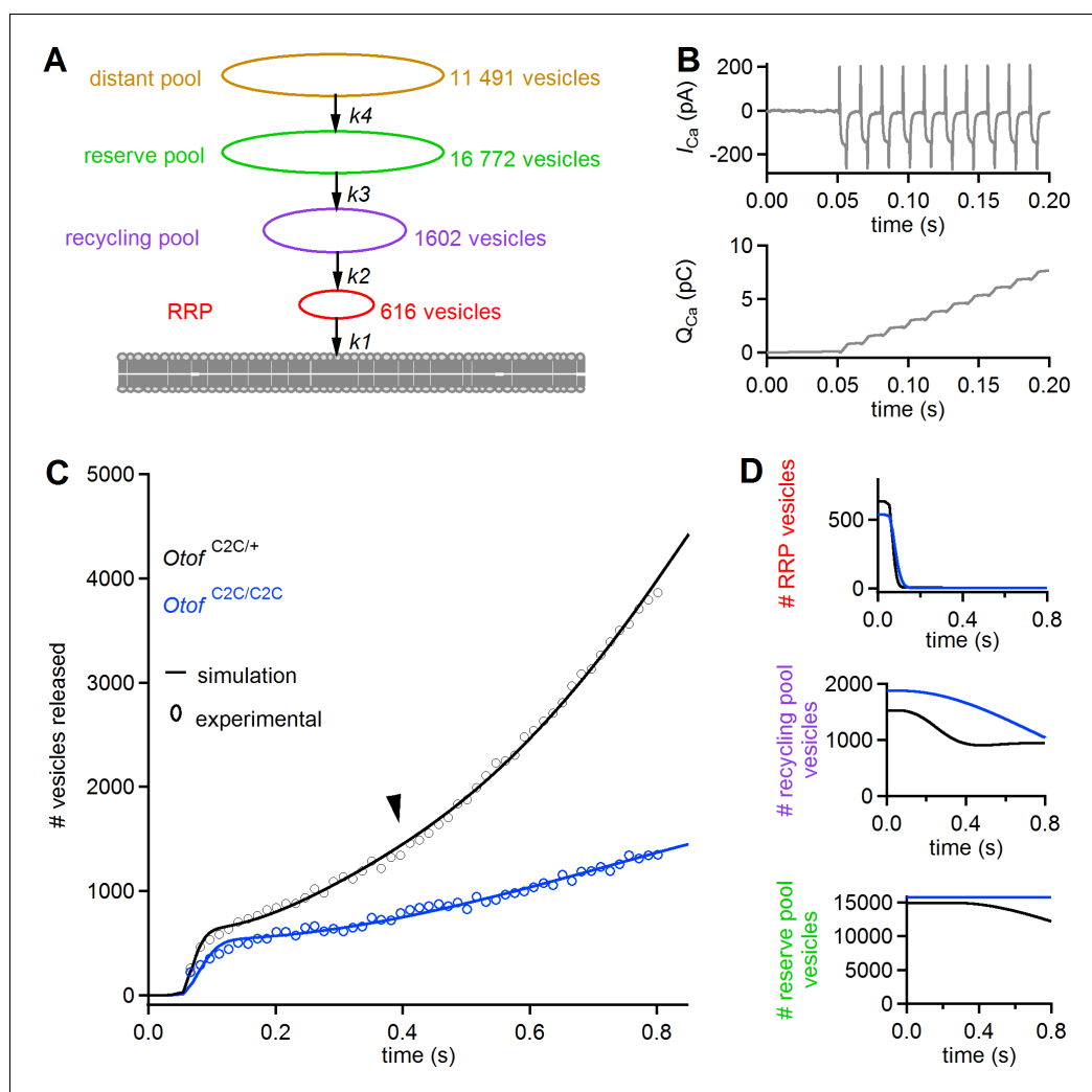
Figure 11. A mass action model of synaptic release reproduces Ca^{2+} sensitivity defects in Otof^{C2C/C2C} IHCs. (A) Diagram of the synaptic vesicle pools described by the model: the RRP (red), the recycling pool (violet), the reserve pool (green), and the distant pool (yellow). The process of synaptic exocytosis is governed by four rate constants, for RRP vesicle fusion ( k_1 ), replenishment of the RRP from the recycling pool ( k_2 ), replenishment of the recycling pool from the reserve pool ( k_3 ), and replenishment of the reserve pool from the distant pool ( k_4 ). The vesicle numbers indicated for each pool are the results obtained by least-squares fitting to the experimental data for Otof^{C2C/+} IHCs. (B) Original Ca^{2+} current ( I_{Ca} ) trace (recorded without the sine wave variation of the holding potential used to determine C_m ) elicited by a train of 50 successive 5 ms depolarizations in an Otof^{C2C/+} IHC (upper panel), and the corresponding integrated charge Q_{Ca} as a function of time (lower panel). (C) Experimental mean \Delta C_m data as in Figure 8F , converted into the number of fused vesicles (black and blue circles) during a train of 50 successive 5 ms depolarizations, superimposed onto the best least-squares fits (black and blue lines) of the model for Otof^{C2C/+} and Otof^{C2C/C2C} IHCs (see Table 1 ). (D) Corresponding simulation of changes in vesicle numbers for each vesicle pool in Otof^{C2C/+} and Otof^{C2C/C2C} IHCs.
