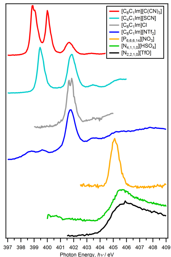
Figure 2. Experimental N 1s edge NEXAFS spectra for seven ILs using partial electron yield (PEY) detection. The features at h\nu < 400 eV for [C_8C_1Im][NTf_2] are most likely due to sample damage (see text). The spectra are vertically offset for clarity.
