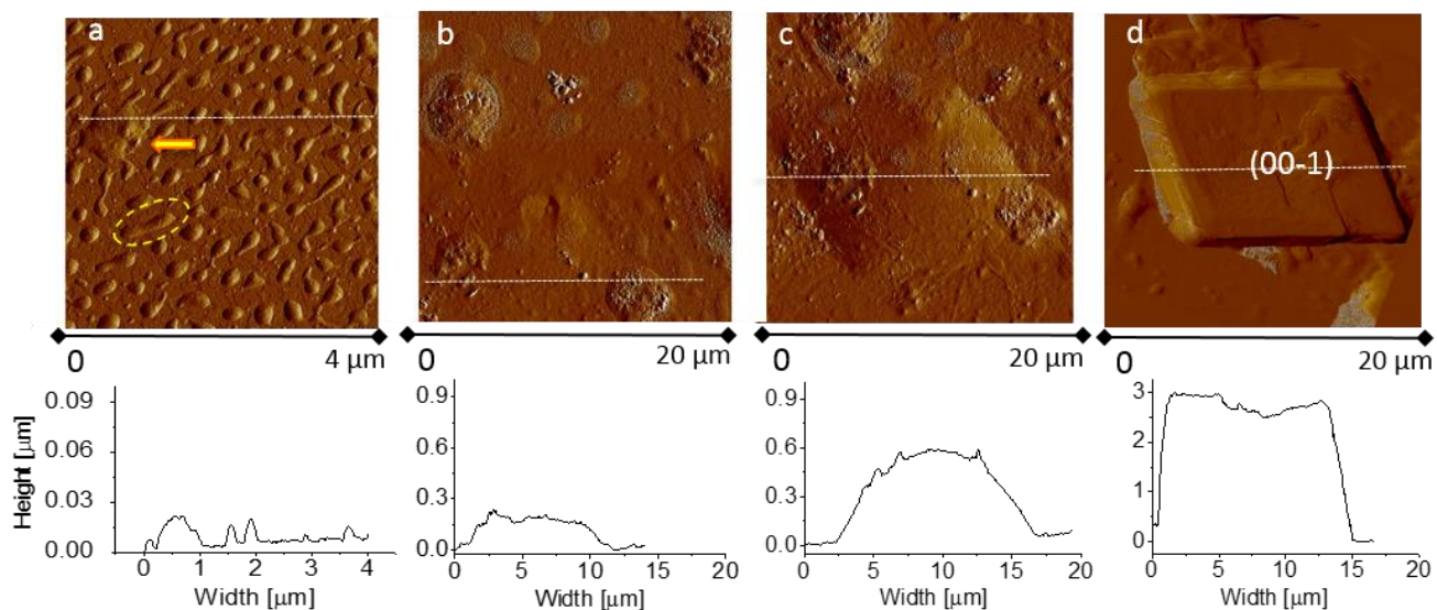
Figure 4 AFM micrographs with the corresponding cross section of height (area marked with dotted white line) of the surface of (100) OZPNI in water showing the evolution of size and ordered features after a) 2 h- visible droplets on the surface, droplet coalescence marked with yellow arrow and two droplets coalescing marked with dashed circle b) 24 h- coalescence of the
