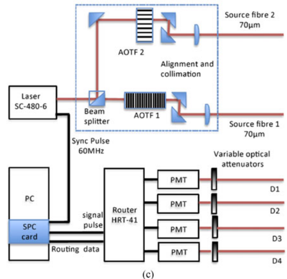
Fig. 1. (a) Picture of the front of the system, (b) Picture of the rear of system, showing fibre optic connections. (c) Schematic illustration of the major system components.
