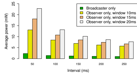
Fig. 4: Average power consumption in isolation by Broadcaster and Observer roles for different combinations of Advertising and Scan Interval (x-axis) and Scan Window (last three colours).
