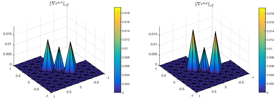
Figure 3: [L-shape problem from Section 6.2] For the three marked vertices in \widetilde{\mathcal{V}}_6^\theta , we display the piecewise \mathbb{P}_1 functions which take the value \|\nabla r^{a,h}\|_{\omega_6^a} in the vertex \mathbf{a} and 0 elsewhere ( left ) and the value \|\nabla r^{a,p}\|_{\omega_6^a} in the vertex \mathbf{a} and 0 elsewhere ( right ).
