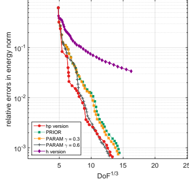
Figure 5: [Sharp-Gaussian of Section 6.1] Relative energy error \|\nabla(u - u_\ell)\| / \|\nabla u\| as a function of \text{DoF}_\ell^{\frac{1}{3}} , obtained using the present hp -decision criterion, the criteria PRIOR and PARAM ( \gamma = 0.3 , \gamma = 0.6 ), and using only h -refinement.
