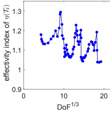
Figure 13: [L-shape domain of Section 6.2] The effectivity indices of the error estimate \eta(\mathcal{T}_\ell) , defined as \eta(\mathcal{T}_\ell)/\|\nabla(u - u_\ell)\| , throughout the 65 iterations of the present hp -adaptive procedure.
