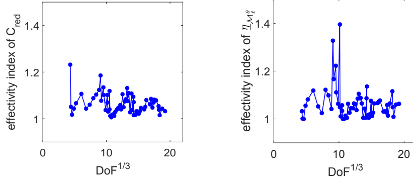
Figure 15: [L-shape domain of Section 6.2] Effectivity indices (6.2) for the error reduction factor C_{\text{red}} from Theorem 5.2 (left) and effectivity indices for the lower bound \underline{\eta}_{\mathcal{M}_\ell^\theta} from Lemma 5.1 defined as the ratio \|\nabla(u_{\ell+1} - u_\ell)\|_{\omega_\ell} / \underline{\eta}_{\mathcal{M}_\ell^\theta} (right).
