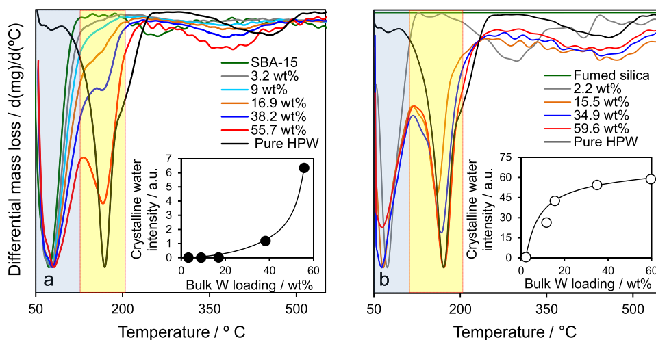
Fig. 4. Differential thermal analysis profiles for (a) HPW/SBA-15, and (b) HPW/fumed silica as a function of bulk W loading. Insets shows integrated desorption peak for crystalline water. (For interpretation of the references to color in the text, the reader is referred to the web version of this article.)
