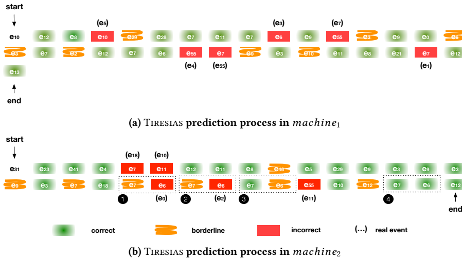
Figure 10: Step by step visualization of TRESIAS prediction process in two real systems. TRESIAS starts with event e_{10} and e_{31} respectively as the initial feed and predicts the upcoming security event step by step. The predictions are colored by their probabilistic scores, where green indicates TRESIAS returns a correct prediction with probabilistic score greater than 0.5, orange indicates TRESIAS returns a correct event prediction with probabilistic score less than 0.5 (but remains the largest probabilistic score), and red indicates a wrong prediction (the actual events are shown in parentheses in this case).
