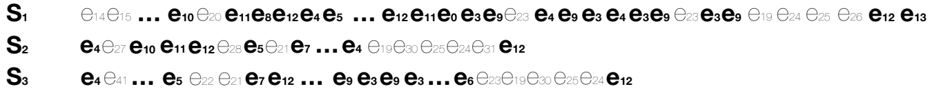
Figure 1: Three endpoints undergoing a coordinated attack. \{e_0, \dots, e_{13}\} are events involved in the coordinated attack and highlighted in bold.
