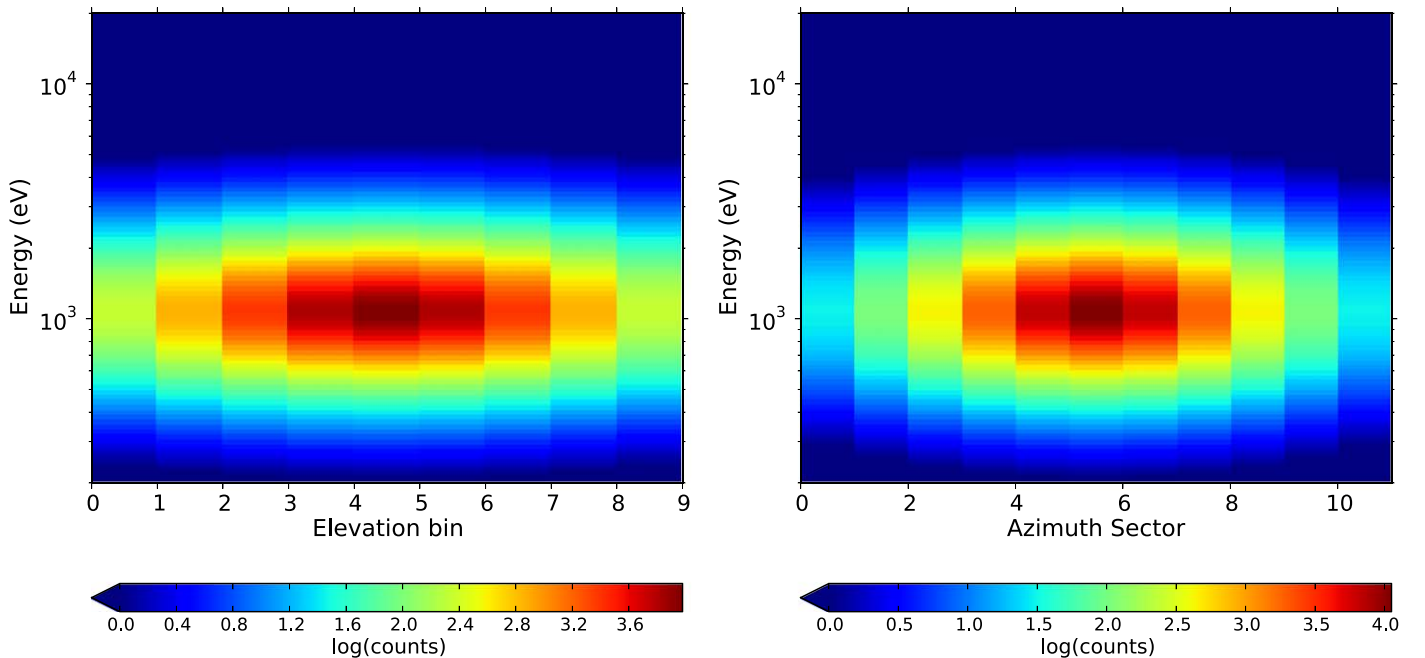
Figure 3. (Left) Elevation-energy matrix and (right) azimuth-energy matrix of SWA-PAS pseudo-observations for protons with bulk energy E_0 = 1 keV, temperature T = 40 eV, and a \kappa = 3 .
