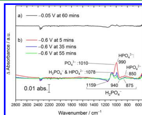
Figure 5. In situ ATR IR difference spectra obtained at the greigite-modified electrode in deoxygenated solution at pH 6.8 0.1 M \text{K}_2\text{HPO}_4/\text{KH}_2\text{PO}_4 at (a) -0.05 and (b) -0.60 V (5 min = red; 35 min = blue; 55 min = green).
