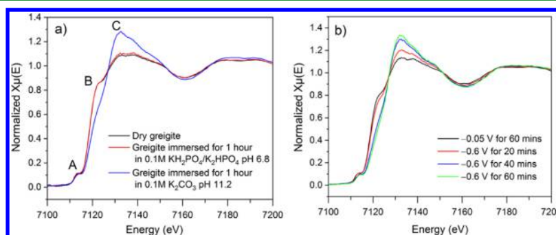
Figure 3. (a) XANES spectra for dry greigite (black); greigite immersed for 1 h in deoxygenated pH 6.8 0.1 M \text{KH}_2\text{PO}_4/\text{K}_2\text{HPO}_4 solution (red) and pH 11.2 0.1 M \text{K}_2\text{CO}_3 solution (blue). (b) XANES spectra for the greigite electrode in deoxygenated pH 6.8 0.1 M \text{K}_2\text{HPO}_4/\text{KH}_2\text{PO}_4 solution at -0.05 V vs SHE for 60 min (black) and -0.60 V vs SHE after 20 min (red), 40 min (blue), and 60 min (green). Labels A–C are described in the text.
