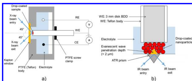
Figure 2. Schemes of (a) in situ XAS electrochemical cell, side view cross section (not to scale). WE = working electrode; CE = counter electrode; RE = reference electrode; (b) in situ ATR IR experiment (not to scale); BDD = boron-doped diamond.
