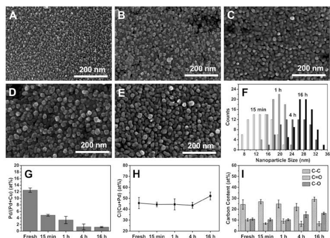
Figure 3. SEM images of (A) a fresh Pd-decorated Cu electrode and Pd-decorated Cu electrodes having performed electrocatalysis for (B) 15 min, (C) 1 h, (D) 4 h and (E) 16 h. (F) Size distributions of the nanoparticles formed on the used Pd-decorated Cu electrodes. (G) Surface Pd/(Cu+Pd) atomic ratios, (H) surface C/(Cu+Pd) atomic ratios and (I) further breakdown of the C content for the fresh and used Pd-decorated Cu electrodes.
