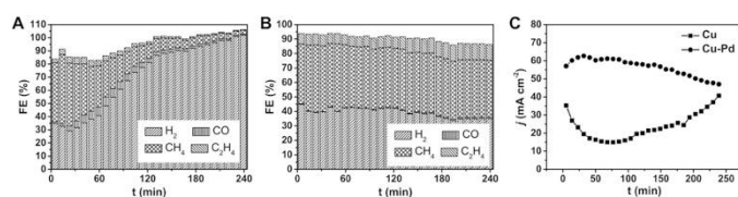
Figure 1. Distributions of gas products as the CO 2 reduction electrocatalysis proceeds on (A) Cu electrode and (B) Pd-decorated Cu electrode, and (C) their time-dependent total current densities at -0.96 V vs RHE in CO 2 -saturated 0.5 M KHCO 3 .
