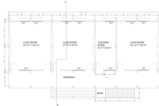
Figure 2: Plan of a prototype Primary School
