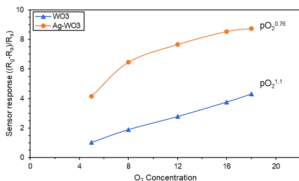
Fig. 8. Sensor responses toward various oxygen concentration.
