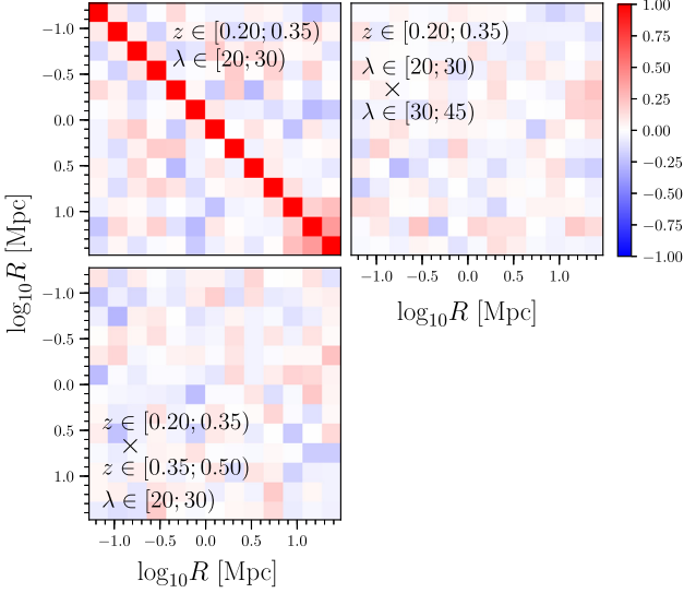
Figure 5. Jackknife-estimated correlation matrix of \widetilde{\Delta\Sigma} of a single richness-redshift selection with \lambda \in [20; 30] and z \in [0.2; 0.35] ( upper left panel ). The off-diagonal blocks display the correlation matrix between the reference profile and the neighbouring richness bin \lambda \in [30; 45] ( upper right panel ), and the neighbouring redshift bin z \in [0.35; 0.5] ( lower left panel ).
