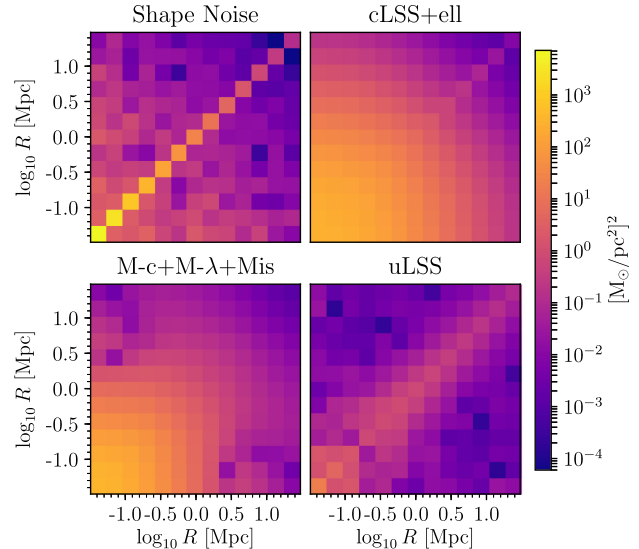
Figure 6. The four individual components to our semi-analytic covariance matrix (SAC). Clockwise from top left: Shape noise component from randomly rotating sources, correlated LSS and ellipticity component from integrating over configurations of the host cluster and its correlated halos, uncorrelated LSS from integrating over large-scale structure, and finally scatter in the M - \lambda relation, M - c relation, and miscentring distribution. Dark colours correspond to low covariance and the colours are log-scaled to show trends. Light colours are normalized to the total covariance in the SAC. See Section 3.2 for details.
