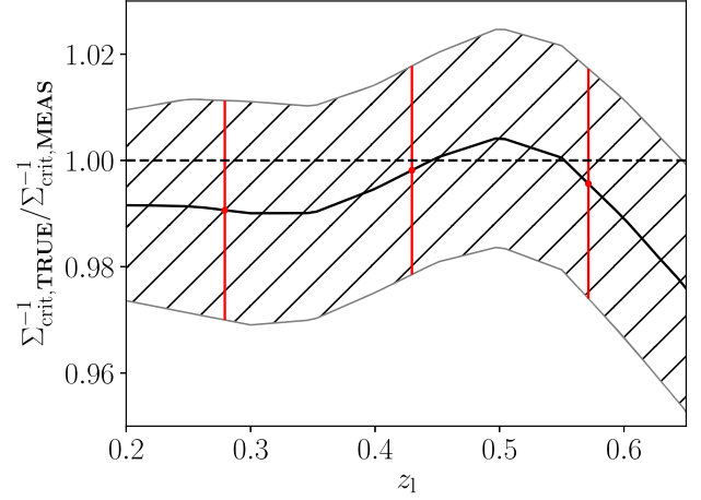
Figure 8. The photo- z correction factor to \Sigma'_{\text{crit}}^{-1} as described in Section 4.3. The grey hatched region indicates the 1\sigma range of the correction factor. Red points with error bars show the correction factors applied to each redshift bin.
