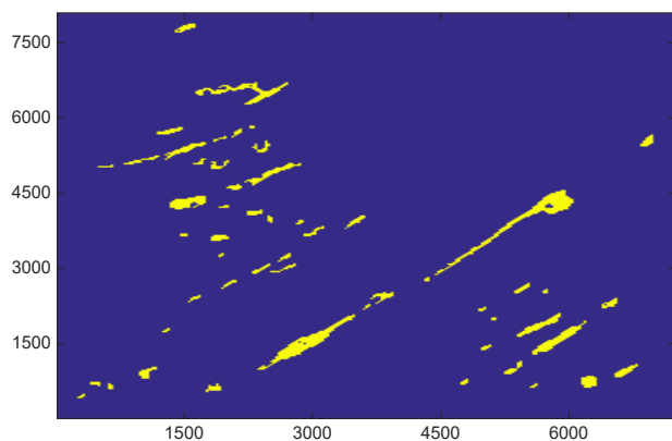
Figure 4. Landsat image of a section of the Larsen C Ice Shelf where melt lakes were present on 6 January 2016. Both axes have units of metres. Here the lakes are coloured yellow and areas where lakes were not present are coloured blue. Although these data were taken from the Landsat 8 mission at a later time than the simulation using the 2010–2011 melt season, it is likely that the lakes will be similar in many aspects due to the role of topography in the location of lake basins. Landsat 8 image courtesy of the U.S. Geological Survey.
