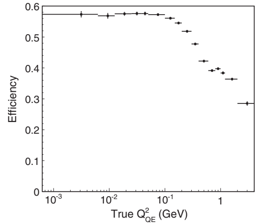
FIG. 22. Selection efficiency for quasislastic-like events in Q_{QE}^2 . The slight increase in efficiency at Q_{QE}^2 0.8 \text{GeV}^2 is due to the proton PID cut definition in Sec. VI A.
