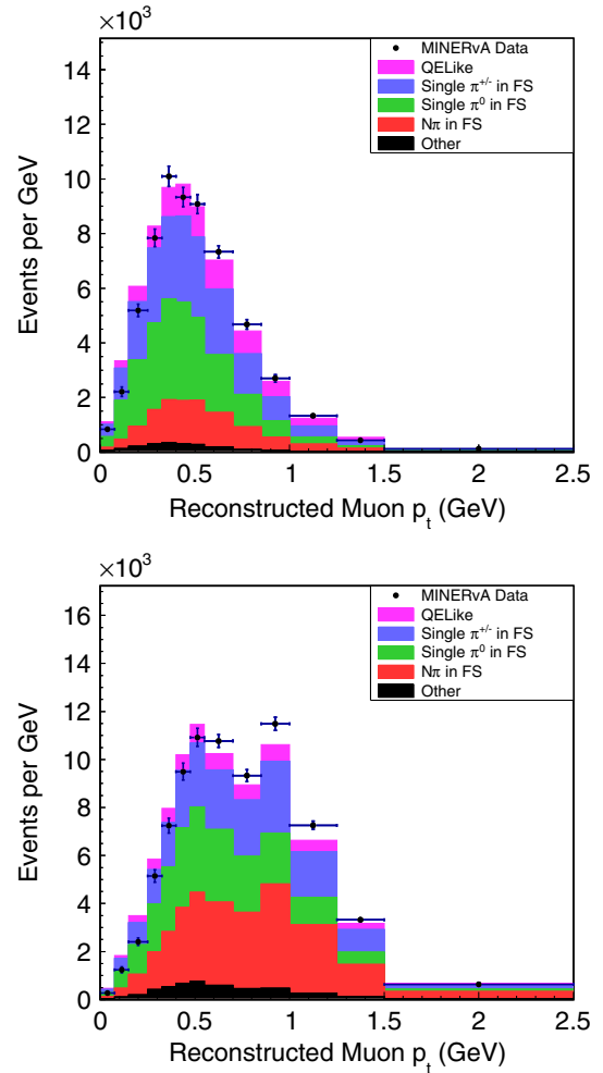
FIG. 12. Control sample containing more than one shower candidate with only the muon reconstructed (top), and with muon and proton candidates reconstructed (bottom).
