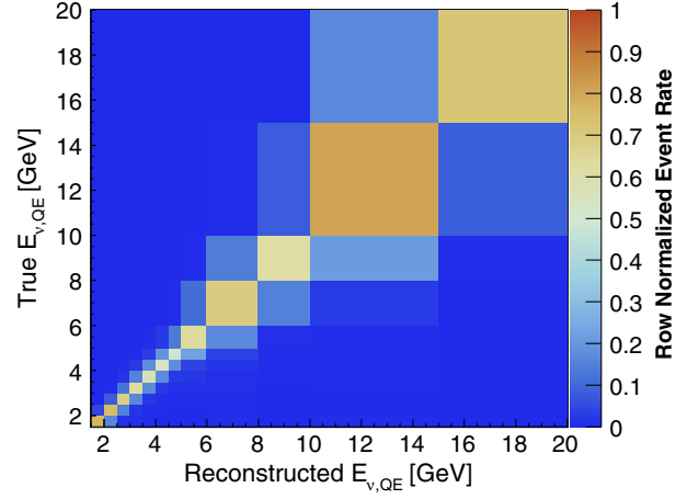
FIG. 18. The migration matrix of E_{\nu,QE} .
