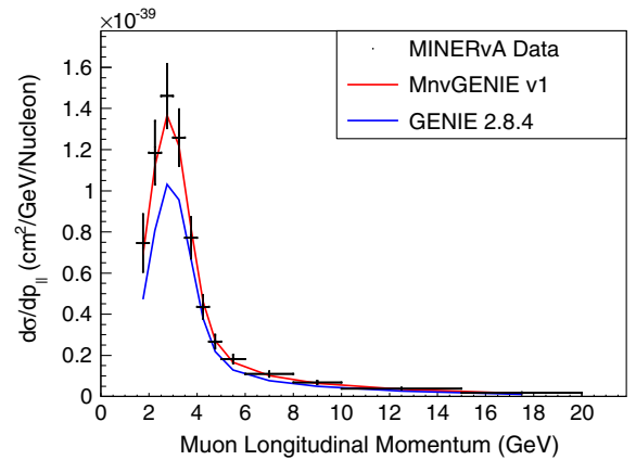
FIG. 43. The differential cross section as a function of p_t and p_{\parallel} with a quasielastic signal definition.
