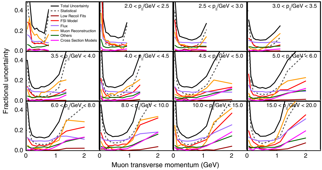
FIG. 45. Systematic uncertainties for the p_{\perp} p_{\parallel} result with a quasielastic signal definition.
