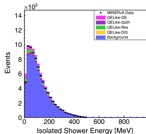
FIG. 7. Energy spectrum of isolated showers.
