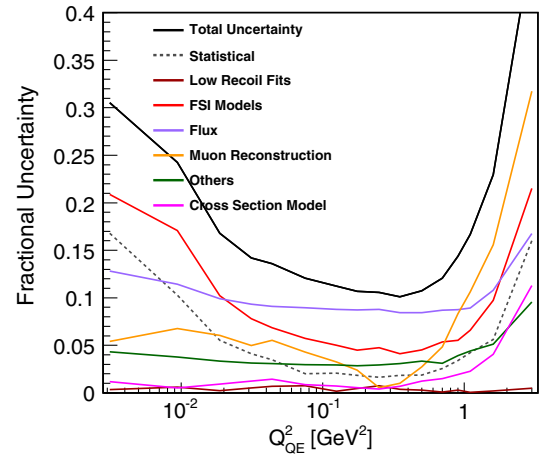
FIG. 47. Systematic uncertainties for the Q_{\text{QE}}^2 result with a quasielastic signal definition.
