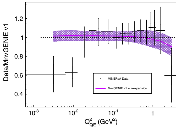
FIG. 42. The differential cross section as a function of Q_{\text{QE}}^2 with a quasielastic signal definition. In addition, the prediction for the z-expansion with the model uncertainty is shown in the ratio.
