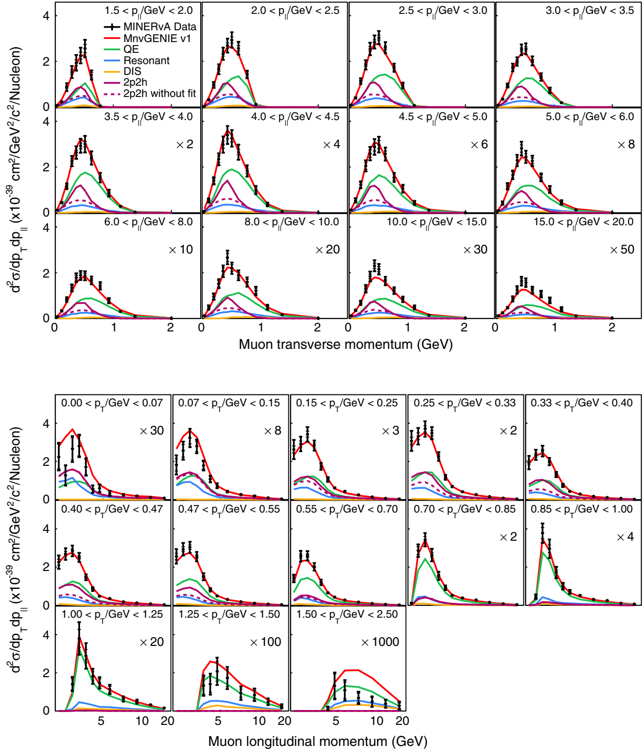
FIG. 27. Full double differential results projected as a function of p_{\perp} and also a function of p_{\parallel} . Unstacked curves show the various components of the MINERvA GENIE tune v1. The dotted line denotes original strength and shape of the 2p2h contribution.
