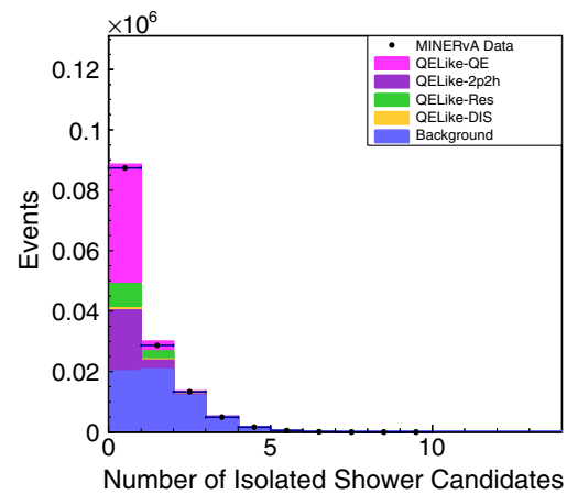
FIG. 5. Number of reconstructed isolated showers.
