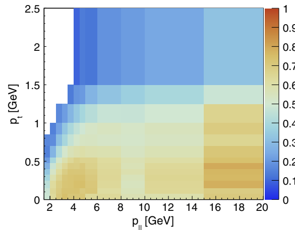
FIG. 20. Selection efficiency for quasielastic-like events.
