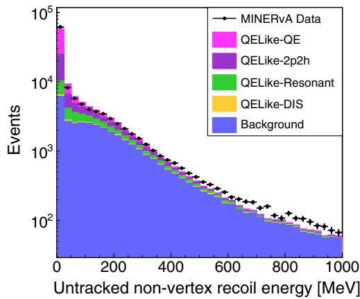
FIG. 4. Recoil spectrum of candidate signal events after all cuts except the recoil cut. The analysis signal is divided up into the initial state processes, as defined by GENIE, include true quasi-elastic events (QELike-QE) and multinucleon effects (QELike-2p2h). The contribution from pion production with subsequent pion absorption (QELike-Resonant and QELike-DIS) is shown. All backgrounds are categorized “Background.”
