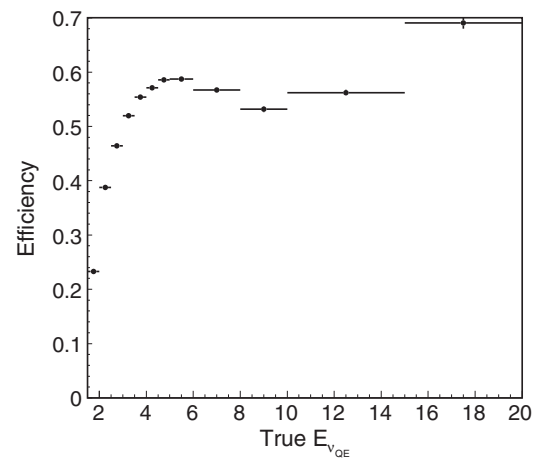
FIG. 23. Selection efficiency for quasislastic-like events in E_{\nu, QE} .
