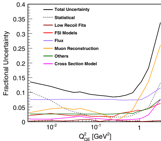
FIG. 25. Systematic uncertainty breakdown for the Q_{QE}^2 result.
