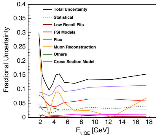
FIG. 46. Systematic uncertainties for the E_{\nu, \text{QE}} result with a quasielastic signal definition.
