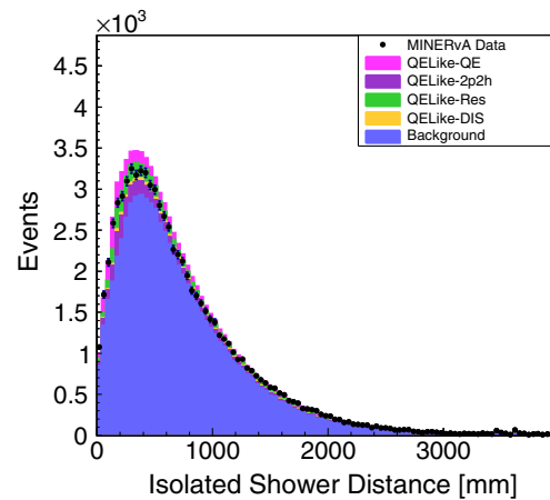
FIG. 6. Distance of isolated showers from the vertex.
