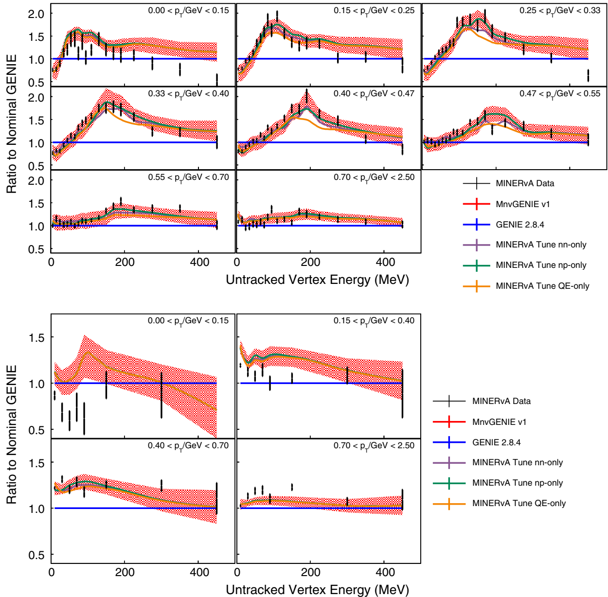
FIG. 39. Vertex energy in p_T bins as compared to variants of the enhancement via 2p2h nn, 2p2h np, or QE only. The single-track (top) and multitrack (bottom) samples are shown. These variations are almost indistinguishable for the multitrack subsample.
