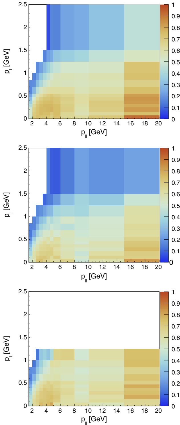
FIG. 21. Selection efficiency for quasislastic-like events broken down by the GENIE component, QE (top), resonant (middle), 2p2h (bottom).
