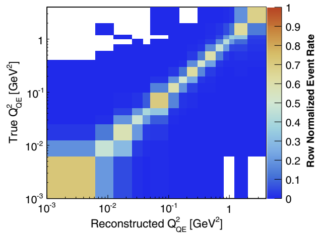
FIG. 19. The migration matrix of Q_{QE}^2 .
