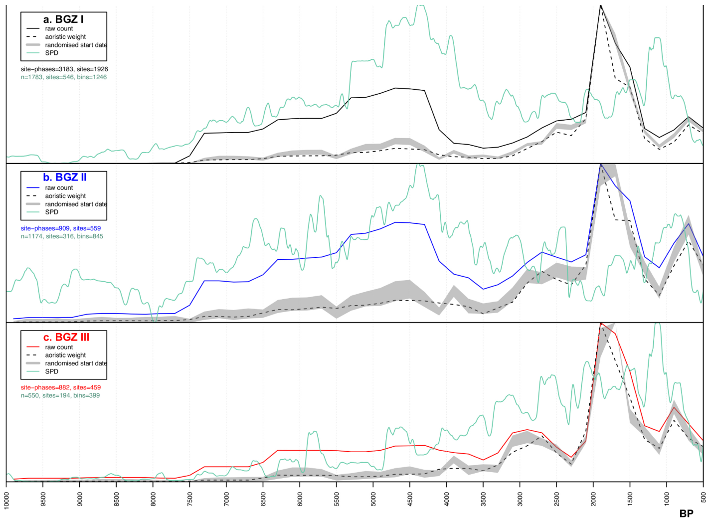
Fig 5 All demographic proxies; a) BGZ I; b) BGZ II; c) BGZ III. Normalised value on a scale between 0 to 1.
