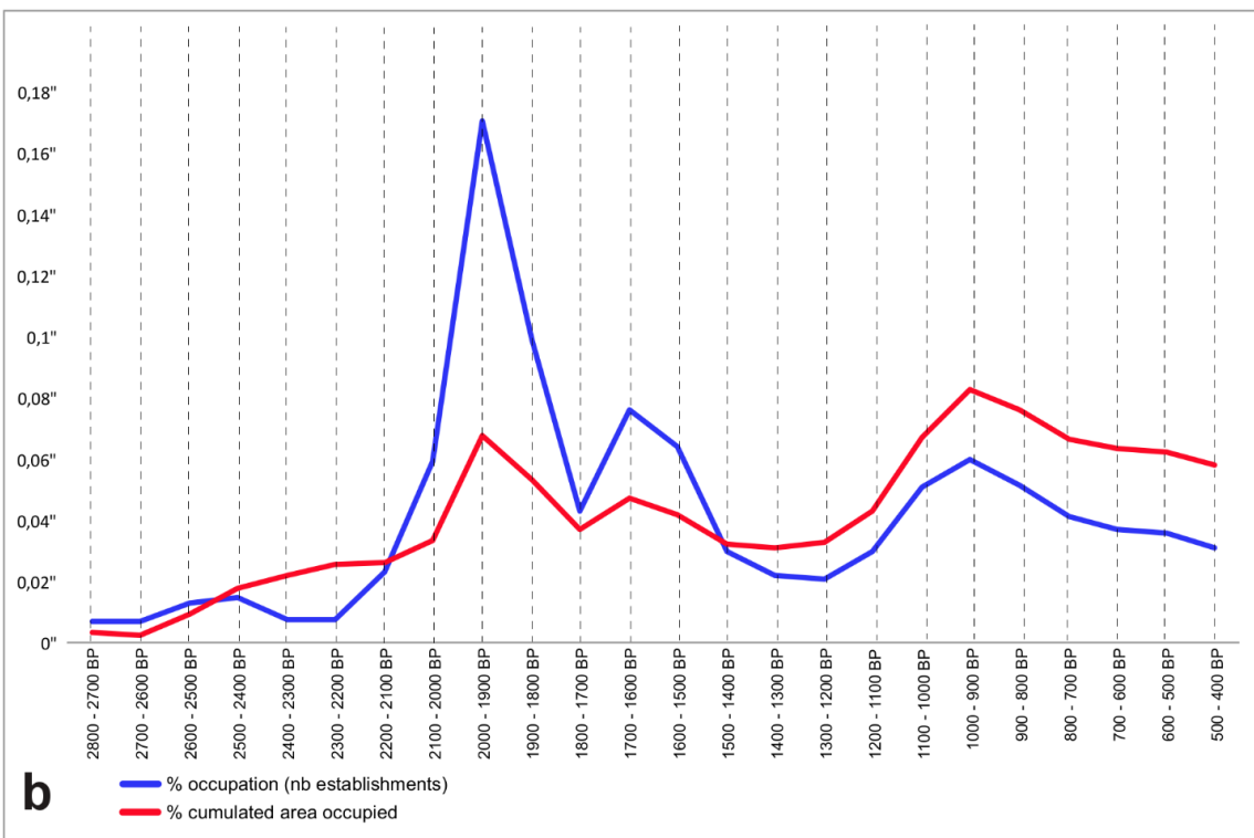
Fig 6a) Site count data for the Eastern Languedoc intensive survey area, comparing the percentage of occupations in each 100 year phase from the Archaeomedes-Archaedyn surveys with the percentage from the same area in the Leverhulme project database; 6b) Site count data for the Eastern Languedoc intensive survey area, comparing the percentage of occupations in each 100 year phase with the percentage of the total area occupied. All data from the Archaeomedes-Archaedyn surveys.
