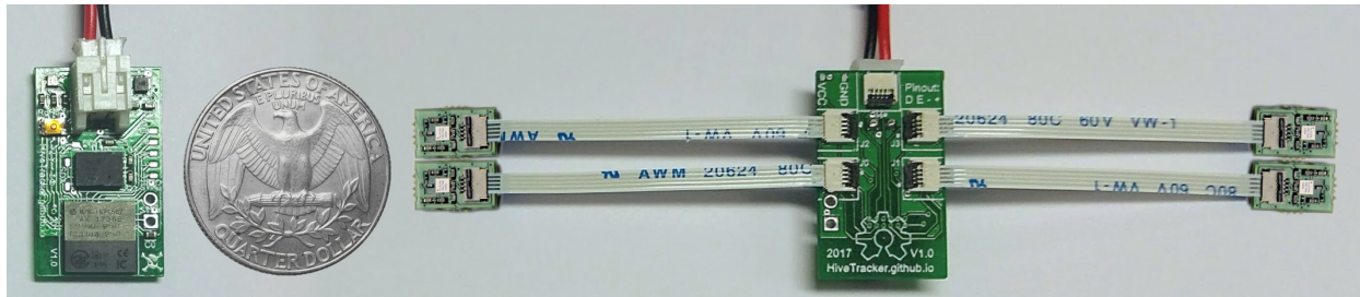
Figure 1: Hive Tracker prototype, with a US 25 cent coin for size comparison.
