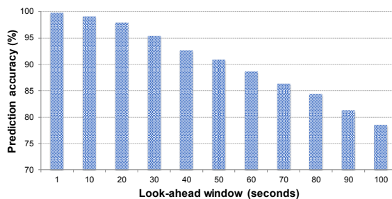
Fig. 10 – Prediction accuracy versus look-ahead window.
