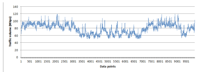
Fig. 9 – Example aggregate traffic trace used for ML training.
