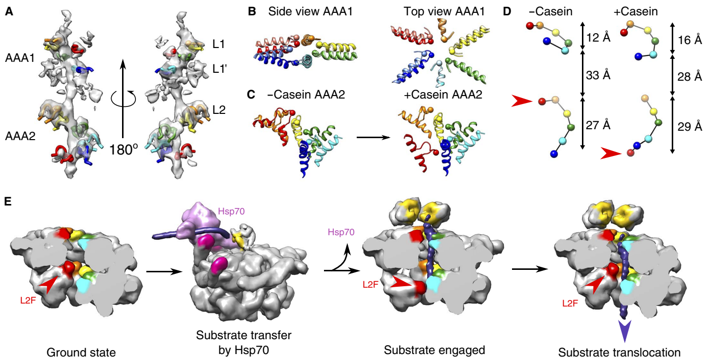
Fig. 4. Track of pore loop interactions with the substrate and movements upon substrate binding. \alpha positions of Tyr 251 and Tyr 653 are indicated by spheres. (A) EM density of the casein substrate and interacting pore loops. Conserved tyrosine pore loops (L1 and L2) and conserved AAA1 loop (L1') form a well-defined spiral track wrapping around the substrate. (B) Conformational changes in tyrosine pore loops of AAA1. Models for ground-state and substrate-bound ClpB are shown in pale and bright colors, respectively. (C) Conformational changes in the tyrosine pore loops of AAA2 and 90° rotation of L2F upon substrate binding. (D) Spiral tracks of tyrosines in ground and substrate-bound states. Red arrowheads indicate the positions of the seam subunit AAA2 tyrosine in the two states. (E) Model of substrate engagement and threading by ClpB. The model was generated using the ClpB models from the present study and a Protein Data Bank (PDB) model of DnaK (4B9Q), docked to motif 2 of a tilted MD of ClpB using available structural information (10). In the case of empty ClpB-ATP- \gamma -S, the position of motif 2 of tilted MDs was extrapolated using the MD conformation of a horizontal MD docked into tilted motif 1.
