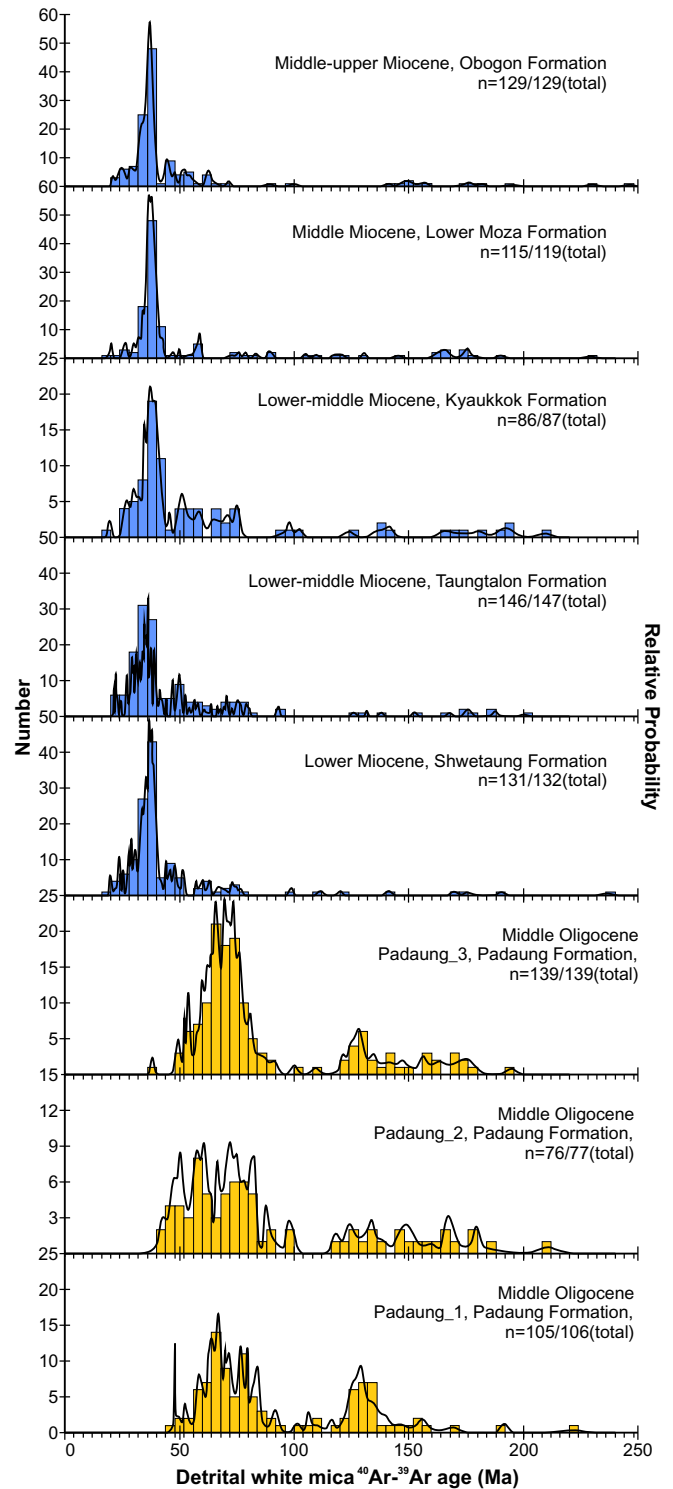
Fig. 15. ^{40}\text{Ar}\text{-}^{39}\text{Ar} data (< 250 Ma) of detrital mica samples from Central Myanmar Basin plotted as relative probability and frequency plots. Data are reproduced from the unpublished PhD thesis of Brezina (2014).
