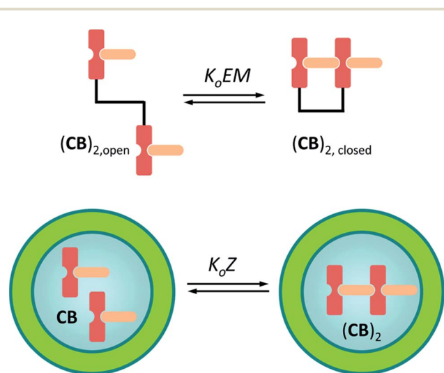
Fig. 6 Top: schematic representation of the equilibria between the open and closed form of an intramolecular (\text{CB})_2 molecule. Bottom: equilibrium leading to the formation of minimal polymer (\text{CB})_2 in the cavity of a vesicle.
