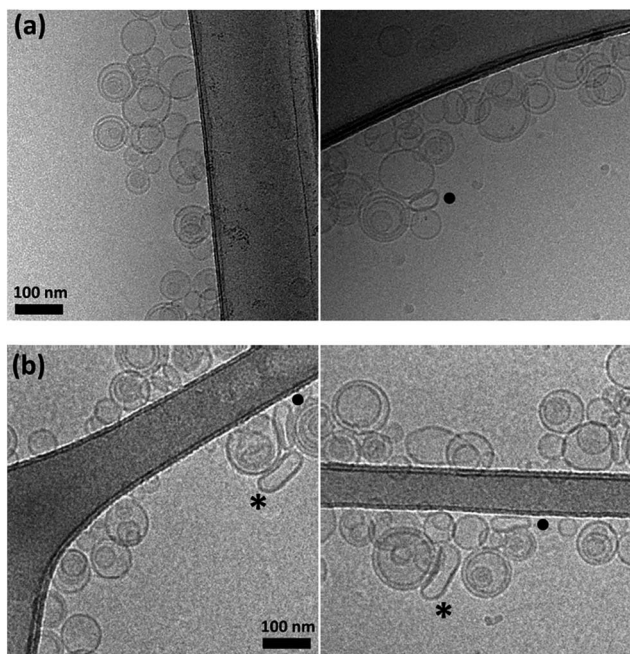
Fig. 8 (a) Detail of a cryo-TEM image of a sample of vesicle-confined C ( [C]_0 = 1.8 \mu\text{M} and [C]_{n0} = 1 \text{ mM} ). (b) Detail of a cryo-TEM image of a sample vesicle-confined C in the presence of B ( [C]_0 = 1.8 \mu\text{M} , [C]_{n0} = 1 \text{ mM} , [B]_0 = 32 \mu\text{M} ). The symbol ( \bullet ) is used to highlight vesicles that appear flattened by the physical constrains imposed by the carbon film support and surrounding vesicles, while ( * ) is used to highlight vesicles that appear flattened without apparent physical constrains.
