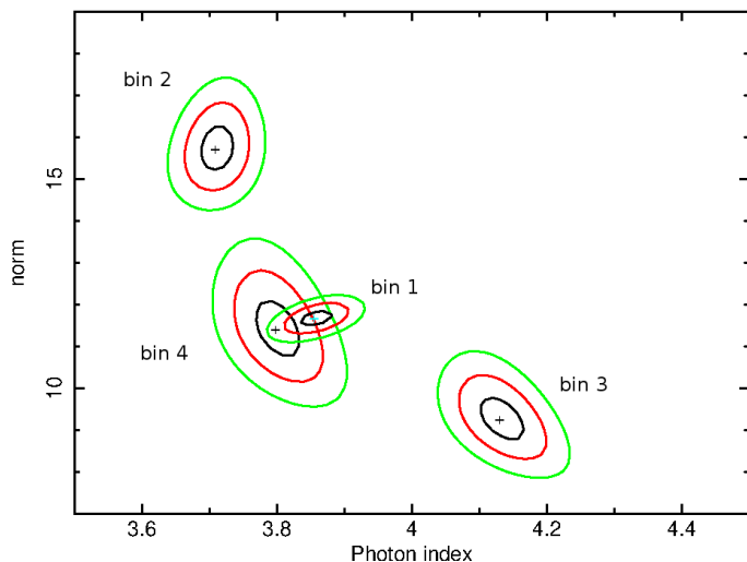
Fig. 8. Contour plots for the 1, 2, and 3\sigma contours of the values of photon index and normalization (unabsorbed flux in the 2–10 keV band in units of 10^{-12} \text{ erg s}^{-1} \text{ cm}^{-2} divided by the constant factors reported in Table 2) of the power-law component of the best-fit model ( \text{const} * \text{gabs} * \text{TBabs} * (\text{pegpwr1w} + \text{bbodyrad}) ) for the four phase bins used in the phase-resolved spectroscopy.
