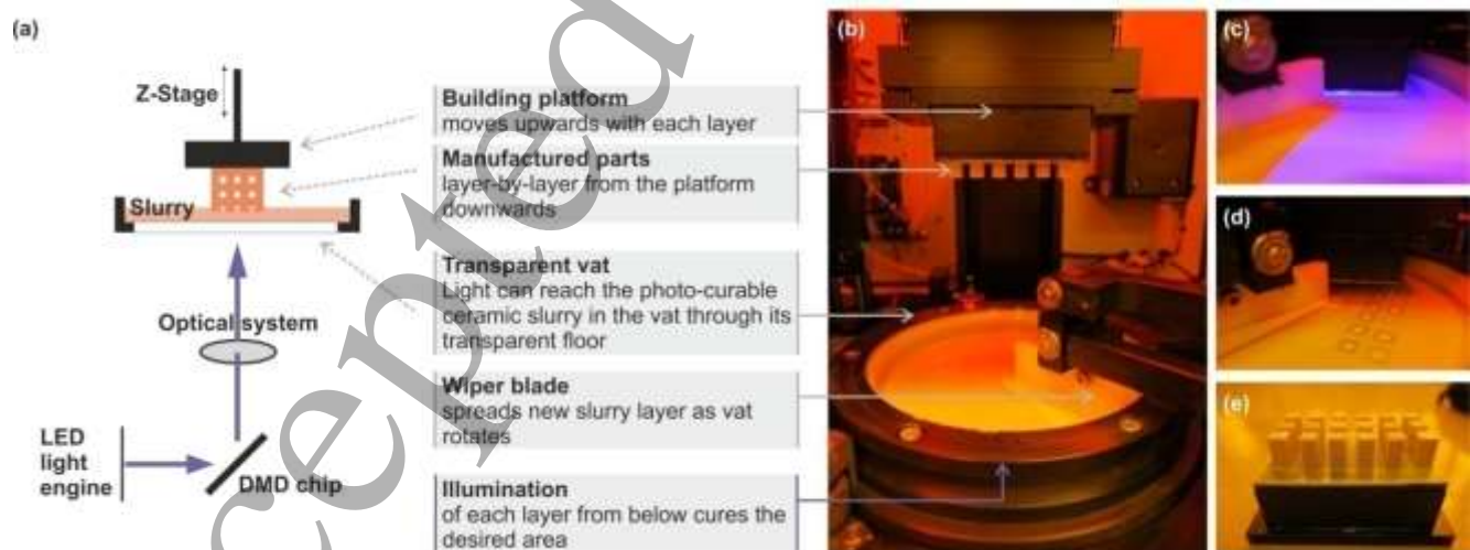
Figure 1: (a): Schematic of a DLP process redrawn from [45]. (b): photographs of the Lithoz CeraFab ceramic additive manufacturing system (LCM); (c): Illumination by DMD from below; (d): lifting-up of the building platform and recoating of the slurry layer; (e): completed green parts still on building platform.
