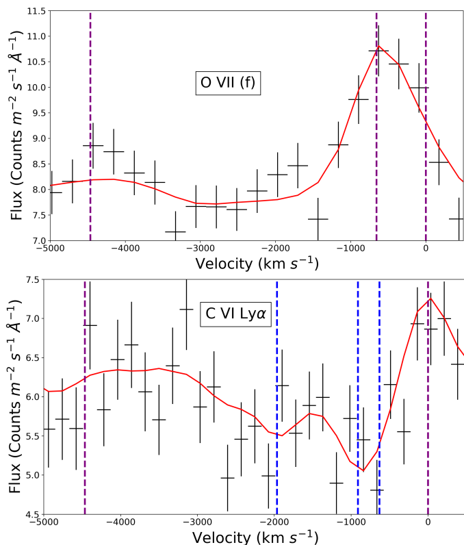
Fig. 4: Velocity plots of the O VII (f) line (top panel) and the C VI Ly \alpha line (bottom panel), illustrating each ion’s velocity profile. Top Panel: The O VII forbidden line is produced by EM1 and EM2 at -657 and 0 km s ^{-1} , respectively, as illustrated by the purple dotted lines showing the outflow velocities of the emission components. EM3 falls at the position of the intercombination line because the forbidden line is blueshifted to higher energies ( v_{out} = 4464 km s ^{-1} ). Bottom Panel: The blue dotted lines indicate the velocities of the three WA components ( v_{out} = -631 , -912 and -1964 km s ^{-1} ) and their contributions to the absorption. The C VI Ly \alpha line is produced at 0 km s ^{-1} , which corresponds to EM2 (purple dotted line). We note that the widths of the emission lines in these two panels are determined fully by the resolution of the RGS instrument ( FWHM \sim 800 km s ^{-1} at 22 Å and FWHM \sim 600 km s ^{-1} at 34 Å, for top and bottom panels respectively), and not by the turbulent velocities ( v_{turb} ) in Table 3.
