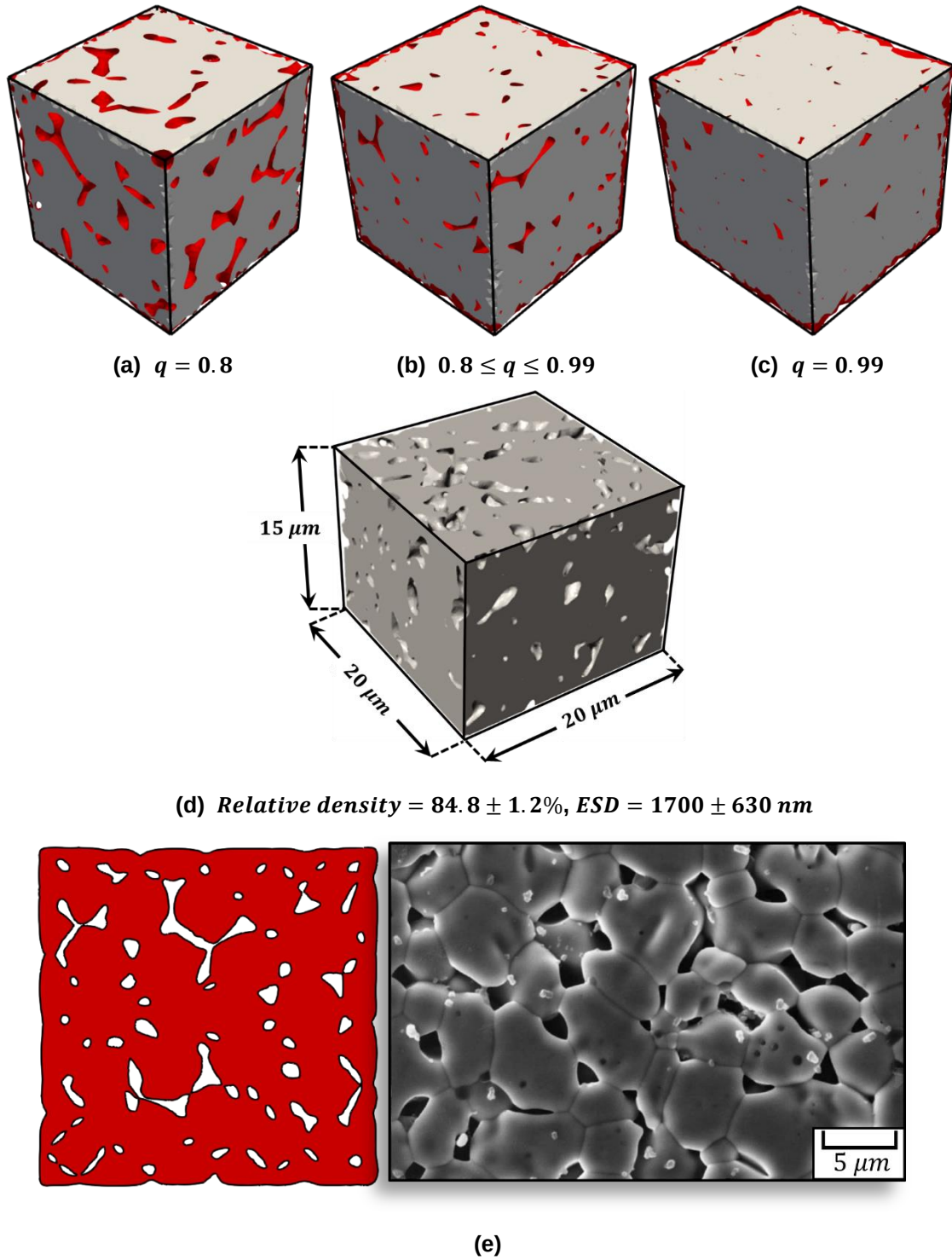
Figure 16. 3D cross-sectional view of three models. Where q = 0.8 , the model includes open porosity (a); by the variable value of q in a range between 0.8 and 0.99, an open-closed porosity is reconstructed (b); and for q = 0.99 , the closed pore system dominates through the structure (c). As an example, the actual digital 3D microstructure of porous LSCF ceramic
