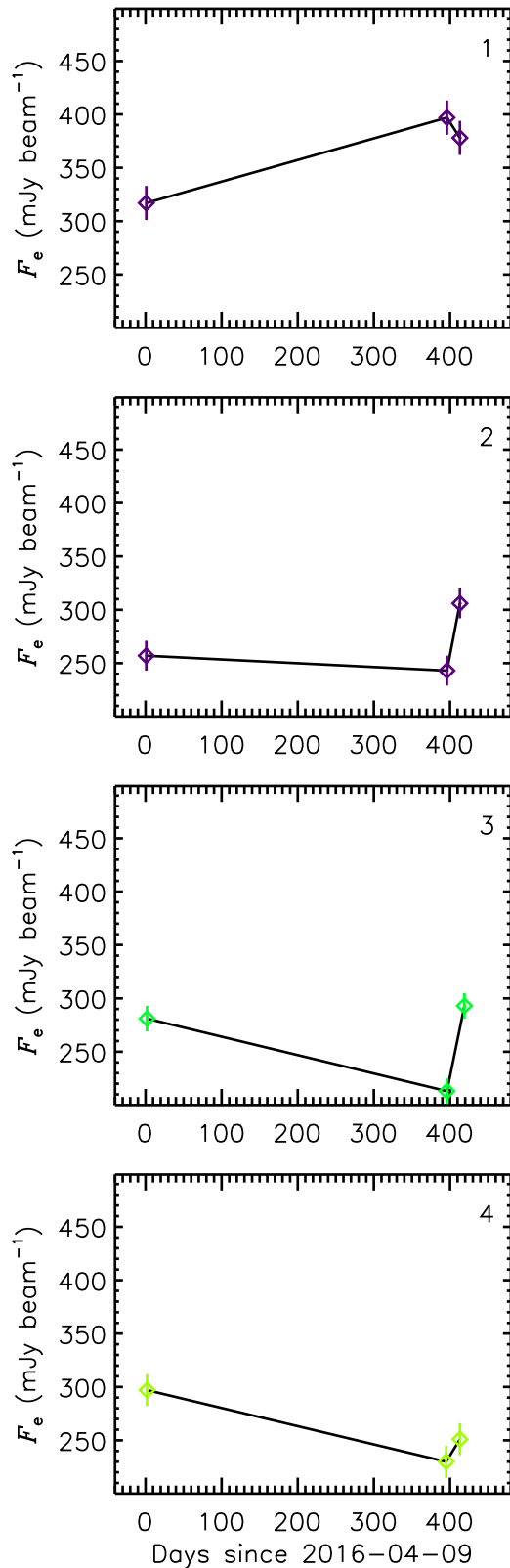
Figure 5. Peak flux variations of the four selected outliers in Table 3. The number assigned to each outlier is written in the top right corner. Symbols and colors are described in Figure 4. The error bars represent \sigma_{\text{std, fid}} .
