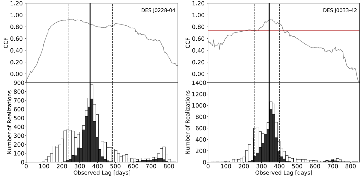
Figure 7. Lag calculations of the two O z DES AGNs. The CCF for each AGN are shown in the top panel . The centroid of the CCF above the red line at 0.8r_{\max} is used to determine the time lag for each realization. The final time lag is the median of the CCCD ( bottom panel ) that is determined using FR/RSS on the light curves with 10 000 realizations. The solid black line represents the measured time lag and the dotted lines mark the 68 per cent confidence levels. The dark grey histogram is the CCCD if we down-weight lags that correspond to light curves with minimal overlap due to the seasonal gaps. The time lags we report are based on the original CCCD (white).
