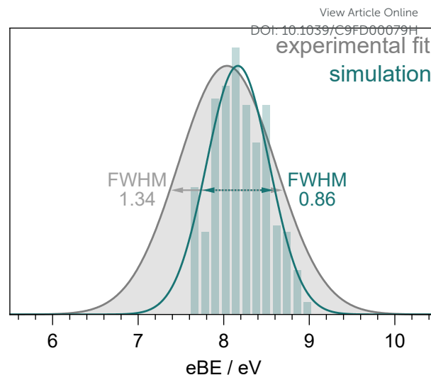
Fig. 5 S_0 - D_0 photoelectron spectra obtained from the fit to the 235.5 nm experimental data (Fig. 3) and simulation (see text). The full-width-half-maxima are shown for both Gaussian fits.
