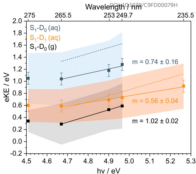
Fig. 4 Plots of fitted Gaussian peak maxima (data points) and full-width half maxima (shaded areas) corresponding to S 1 ( 1^1\pi\pi^* )-D 0 in the gas phase (g) and S 1 ( 1^1\pi\pi^* )-D 0 /D 1 in aqueous solution (aq), as a function of photon energy (bottom axis) and wavelength (top axis). Solid straight lines are fits to the higher photon energy data points, with gradients m indicated. Dashed lines are peak maxima estimated using S 0 -D 0 /D 1 VIEs obtained from X-ray PES 43 and the S 0 -S 1 ( 1^1\pi\pi^* ) AEE determined from the uv-vis absorption spectrum (Fig. 1, orange dashed line), assuming that vibrational energy is conserved during photoionisation.
