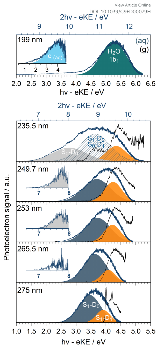
Fig. 3 MPI photoelectron spectra of phenol in the gas phase (black) and in aqueous solution (blue) recorded following photoexcitation at 275 nm (4.51 eV), 265.5 nm (4.67 eV), 253 nm (4.90 eV), 249.7 nm (4.97 eV), 235.5 nm (5.26 eV) and 199 nm (6.23 eV), plotted as a function of one-photon eBE (lower axes). The additional scales marked on the top horizontal axes of the 235.5 nm and 199 nm spectra (blue) represent the two-photon eBEs for these photon energies. Intensities of the individual spectra have been normalised to their maxima. Gaussians represent S_1(1^1\pi\pi^*)-D_0 (dark blue), S_1(1^1\pi\pi^*)-D_1 (orange), S_0-D_0 (light grey). Insets in 265.5-249.7 nm spectra are residuals of the fits of Gaussians to the low eBE edges of the photoelectron spectra, corresponding to S_0-D_0 . The S_0-D_1 ionisation process overlaps with the S_1(1^1\pi\pi^*)-D_0 process in the 235.5 nm PES (stripes). The dark green Gaussian in the 199 nm photoelectron spectrum corresponds to two-photon ionisation from the 1b_1 molecular orbital of H_2O(l) and the inset corresponds to the residual of the low eBE edge (plotted as a function of one-photon eBE) and is attributed to e^-(aq) \rightarrow e^-(g) .
