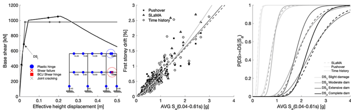
Figure 4: Comparison of the different analysis approaches for the “Pre-Code” building with jacketing.
