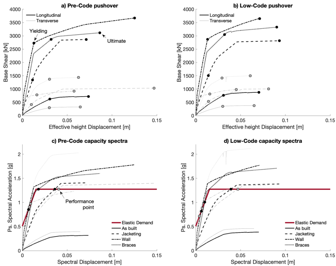
Figure 3: Pushover curves (a,b) and capacity spectra (c,d) for each retrofit solution.
