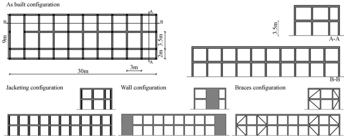
Figure 2: As built and retrofitted configurations for the index building(s).
