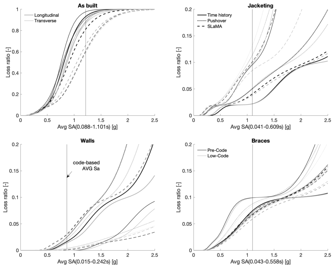
Figure 5: Vulnerability curves for each retrofit solution and analysis method.
