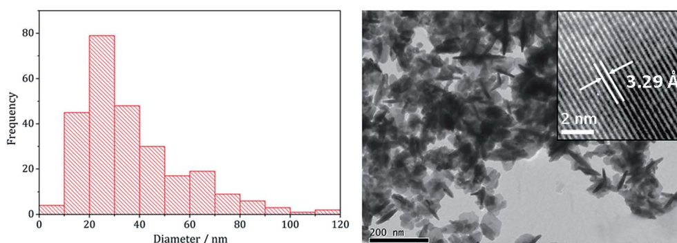
Fig. 4 Particle size histogram (left) and TEM image with HRTEM insert (right) of the \text{FeNi}_2\text{S}_4 sample prepared from mixtures of 1–3 at 230 °C.
