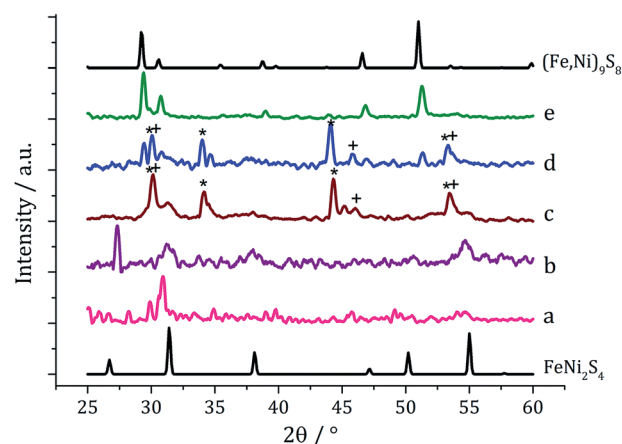
Fig. 1 PXRD patterns for samples prepared from 1 with 2 at (a) 150 °C, (b) 180 °C, (c) 230 °C, (d) 260 °C and (e) 280 °C, with reference patterns for FeNi 2 S 4 (ICDD card no. 47-1740) and (Fe,Ni) 9 S 8 (ICDD card no. 75-2024). '*' indicates Fe 7 S 8 peaks and '+' indicates α-NiS peaks.
