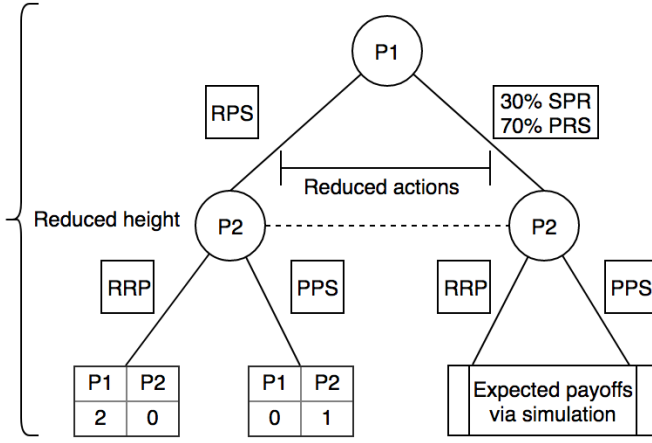
Fig. 2. EGTA-abstracted game for a 2-player-3-round rock-paper-scissors game: each round victory is rewarded with 1 point and draws give no points to either player.
