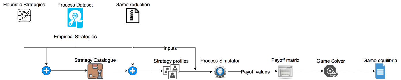
Fig. 3. TASKASSESSOR: Empirical game design for modelling software processes.
