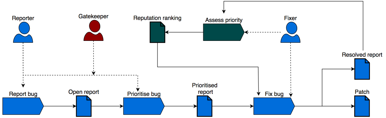
Fig. 4. Bug prioritisation processes: The blue components are shared between the three processes (including distributed prioritisation), the red ones are exclusive to the gatekeeper process and the green ones to the assessor-throttling process. The solid lines represent the input/output of an activity, and the dashed lines link an activity with its performing role.
