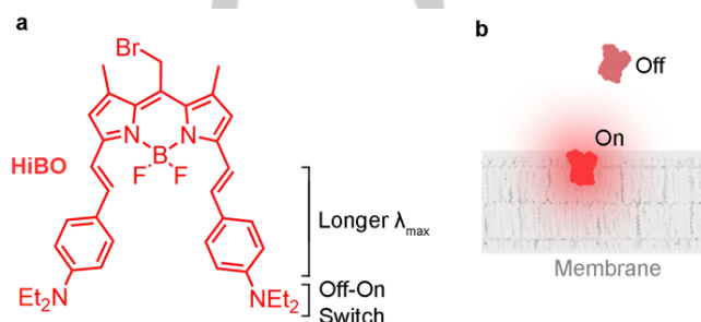
Figure 3. Principle mechanism of environmentally-sensitive membrane fluorophore HiBO, its structure and synthesis. a) Near infra-red fluorophore HiBO highlighting the principles that guided its rational design. b) Schematic representation of the environmentally dependent activation of the fluorophore upon insertion into a lipid bilayer.
