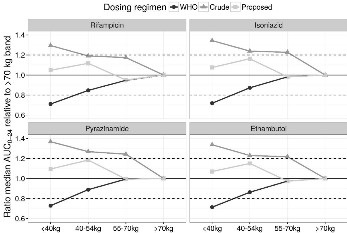
Figure 3. Comparison of predicted relative variability in median exposure across the trial population following proposed adjusted dosing regimens (closed squares) versus regimens based WHO recommended weight band (closed circles) and cut-off value of 50 kg (closed triangles). Patients in the highest WHO weight band (>70 kg) were selected as the reference population. Dashed horizontal lines represent the variability acceptance interval (80-120%).
