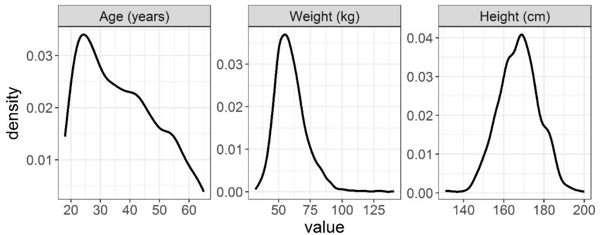
Figure 1. Density plots of the baseline demographic characteristics of the trial population (N=2231). Height distribution was available from 1833 patients only.
