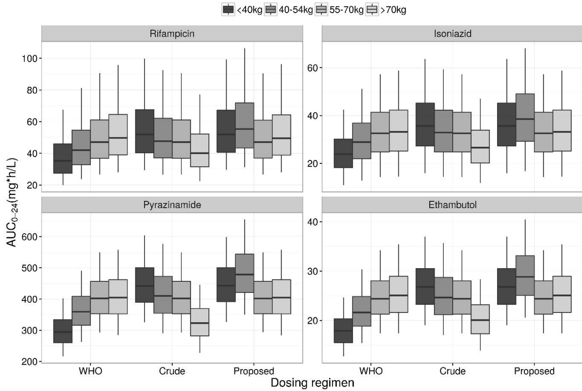
Figure 2. Comparison of simulated AUC_{0-24} at steady state following proposed adjusted dosing regimens versus regimens based WHO recommended weight band and cut-off value of 50 kg (N=2231; 200 clinical trial simulations). Box-plots depict 5 th , 25 th , median, 75 th and 95 th percentile of simulated secondary PK parameters.
