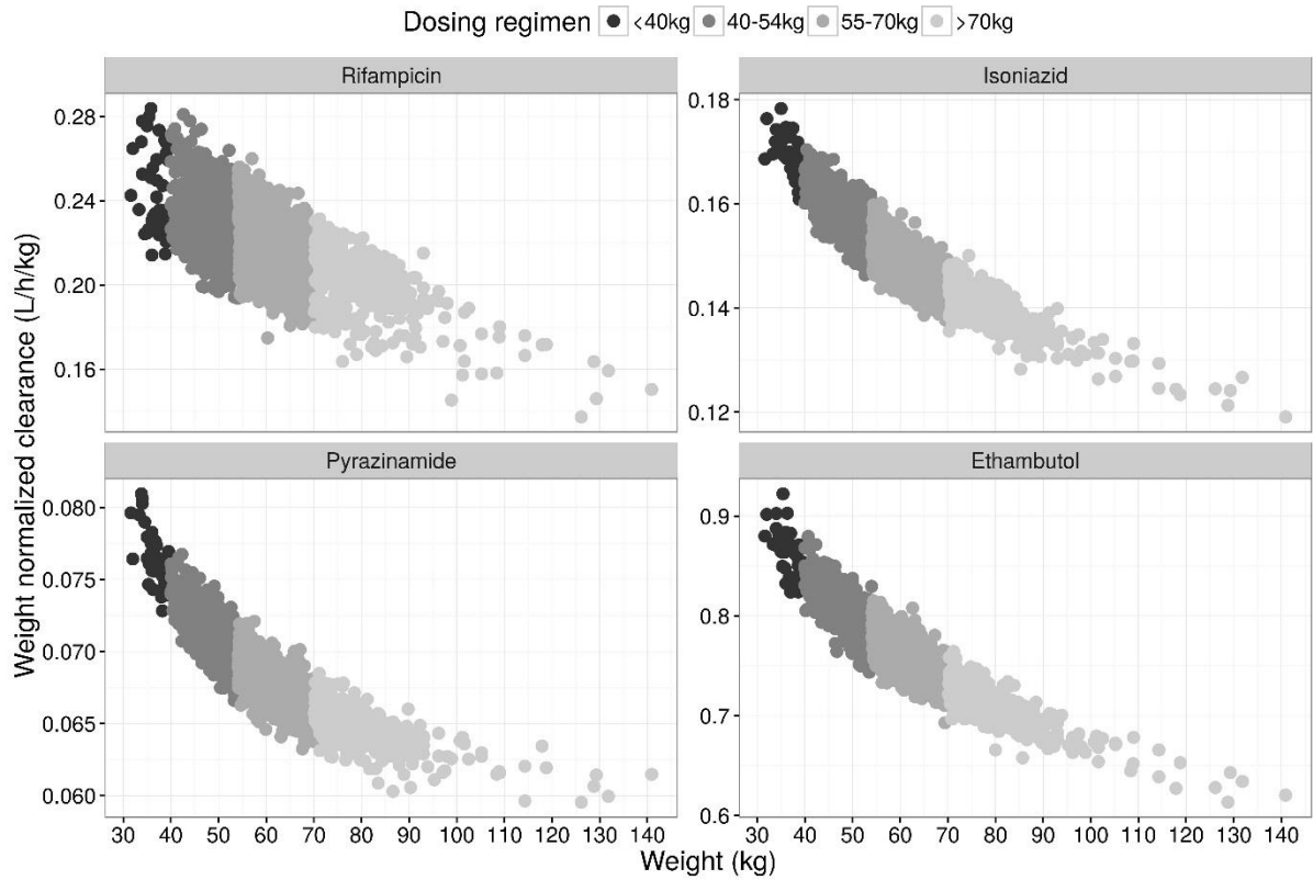
Figure 4. Predicted non-linear relationship between weight and clearance (CL/F) of the standard of care drugs in the trial population (N=2231). Closed circles represent the simulated median individual CL/F, normalized to body weight.
