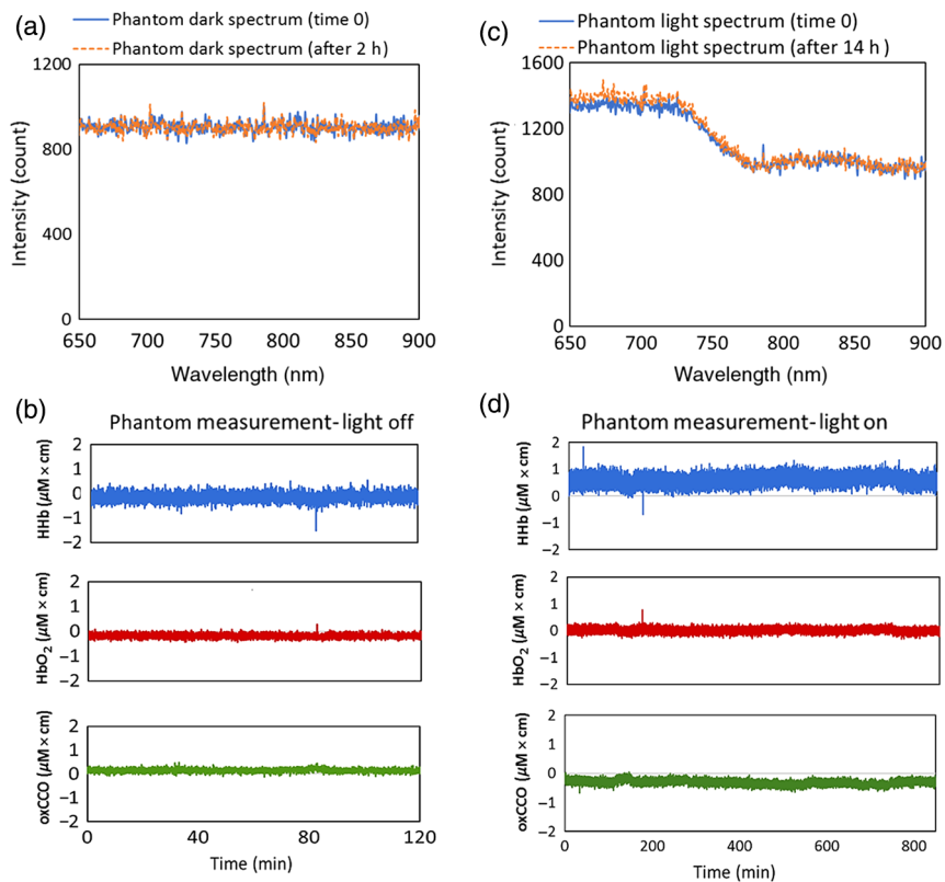
Fig. 6 Phantom measurements in dark and light showing the stability of the miniCYRIL system. (a) and (b) The spectral data and concentration changes in a tissue-like phantom ( \mu_a = 0.02 and \mu'_s = 0.9 , [\text{mm}^{-1} \text{mol}^{-1}] ) for 2 h when the shutter of the light source is closed. (c) and (d) The spectral data and concentration measurements for 14 h, when the same phantom is illuminated (shutter open). Integration time for both measurements is 1 s and SDS is 4 cm.
