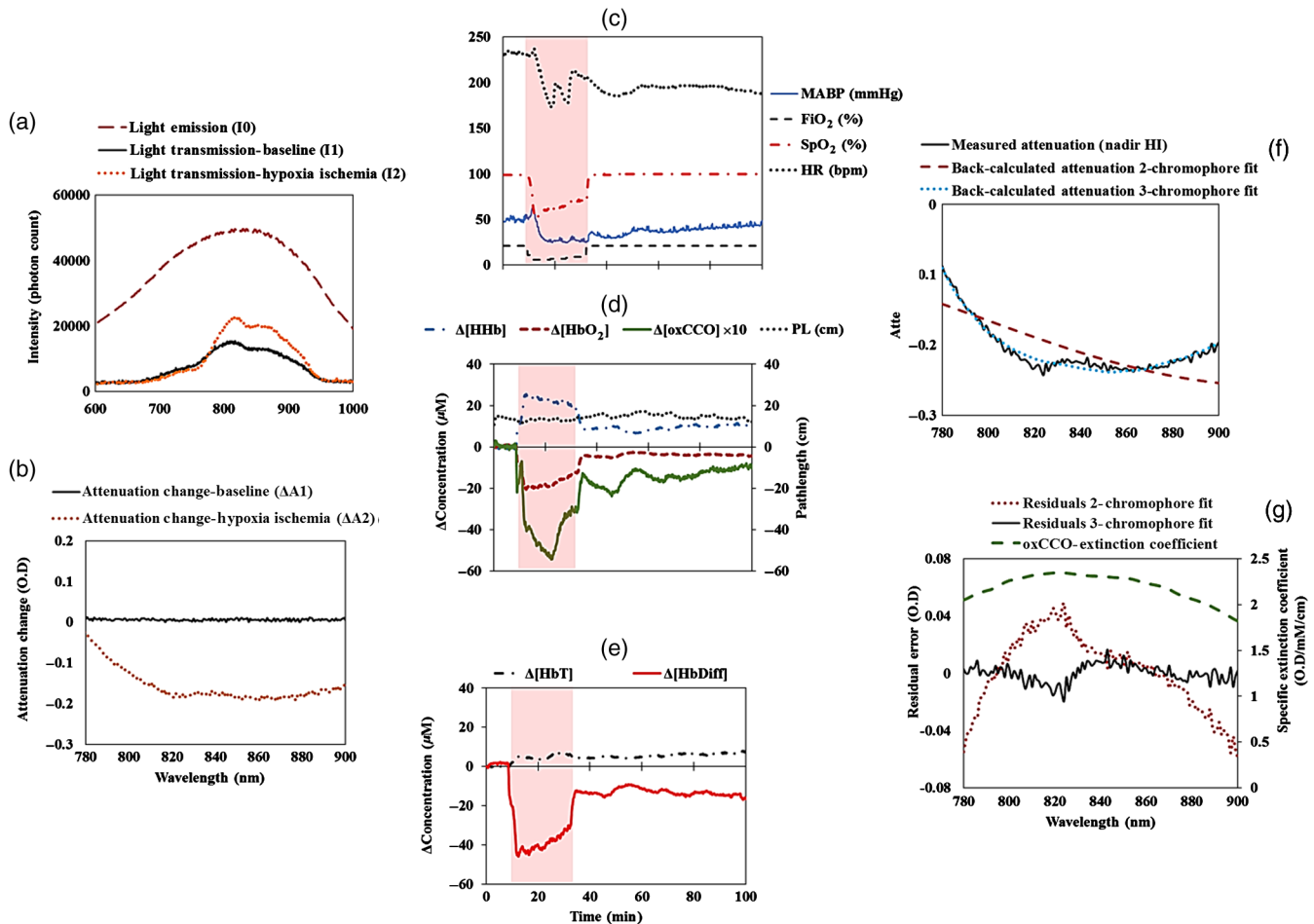
Fig. 2 An example of the optical data from a piglet (LWP483). (a) Incident ( I_0 ) and transmitted light spectra ( I_1 and I_2 ) through the brain during baseline and HI. The significantly reduced photon count in I_1 and I_2 is due to the optical properties of the piglet brain. The increased peak count in I_2 relative to I_1 is due to less absorption during HI. (b) Attenuation spectra measured at baseline and insult. There is no major change in the attenuation spectrum relative to the first measurement at baseline ( \Delta A1 ). However, during HI, there is a significant change in the magnitude and the shape of the attenuation spectrum due to the physiological changes in the brain, i.e., reduction in blood flow and oxygenation ( \Delta A2 ). (c) Changes in the systemic physiological data at baseline, HI, and recovery. (d) and (e) Changes in the bNIRS measurements baseline, HI, and the recovery period as measured by miniCYRIL based on second derivative spectroscopy for pathlength change measurement. The shaded area indicates the HI period. There is no change in the optical pathlength during HI and recovery. (f) Measured attenuation spectrum at HI and back-calculated attenuations from two- and three-chromophore fit. (g) Residual errors from two- and three-chromophore fit residual is similar to the extinction coefficient of oxCCO, whereas the three-chromophore fit residual error is approximately zero.
