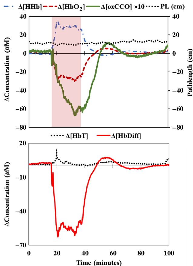
Fig. 8 An example of changes in the bNIRS measurements during baseline, HI, and recovery in a piglet (LWP498) as measured by miniCYRIL based on the second derivative spectroscopy technique for pathlength change measurement. The shaded area indicates the HI period. There is no change in the optical pathlength during HI and recovery. In this piglet, the HbDiff and oxCCO signals demonstrate a hyperemia and hyperactivation phase after HI (above baseline).
