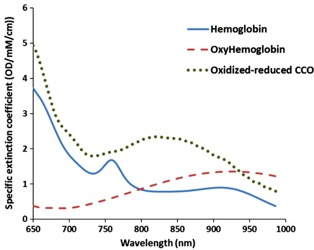
Fig. 7 The specific extinction coefficient of oxygenated and deoxygenated hemoglobin as well as the difference absorption spectrum of oxidized and reduced CCO. The data are taken from Ref. 71.
