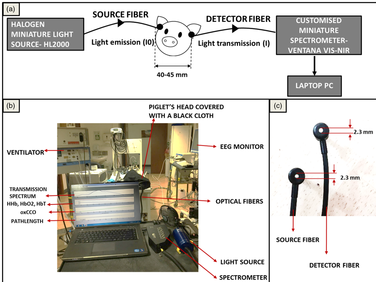
Fig. 1 miniCYRIL setup in a preclinical study of neonatal HIE. (a) A schematic diagram of the experimental design. (b) miniCYRIL's components including a miniature white-light source (HL2000-HP), a customized Ventana VIS-NIR miniature spectrometer, optical fibers, and a laptop for the real-time display of concentration data. Light from the halogen light source is emitted onto the piglet brain ( I_0 ) through a 0.57-NA optical fiber with 2.3-mm diameter (c). Light transmitted through the brain ( I ) is collected at tissue surface (SDS: 40 to 45 mm) through an identical optical fiber and transferred to the miniature spectrometer. A MATLAB program then converts the collected spectral data to changes in attenuation and accordingly calculates changes in the concentration of HHb, HbO 2 , and oxCCO based on the measured optical pathlength. The spectral and concentration data are displayed in real time on a laptop screen (b) and saved in a CSV file after each measurement.
