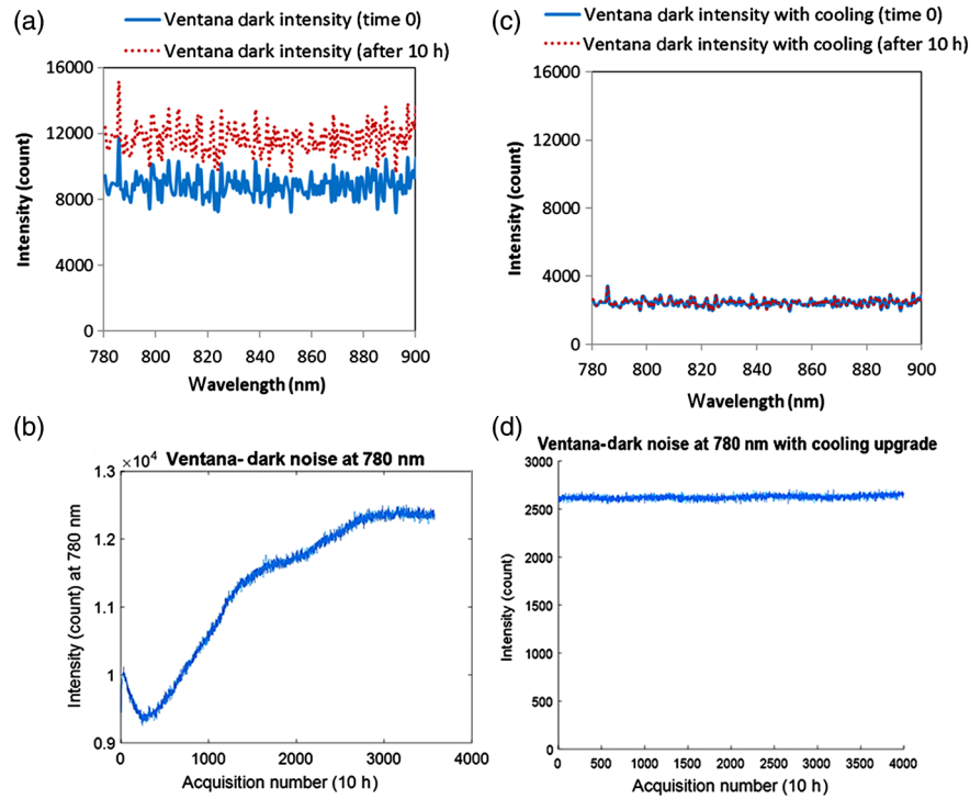
Fig. 5 (a) Dark intensity spectrum measured across 780 to 900 nm every 10 s when the slit of the spectrometer is closed at time 0 and after 10 h. (b) The dark intensity changes at wavelength 780 nm over 10 h. (c) Dark intensity spectrum measured across 780 to 900 nm every 10 s with the upgraded unit, the slit is closed at time 0 and after 10 h. (d) The dark intensity changes at wavelength 780 nm over 10 h.
