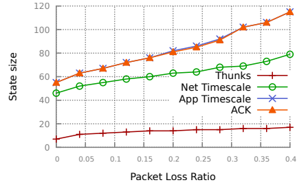
Figure 16: Forwarder state size.
