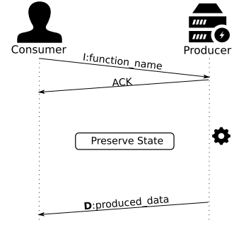
Figure 7: Acknowledgements. The Interest Lifetime is set based on network RTT estimation. The returning ACK inflates PIT expiry timer to match estimated computation time.
