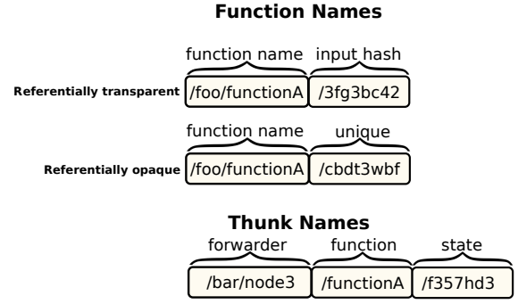
Figure 1: Naming convention.
