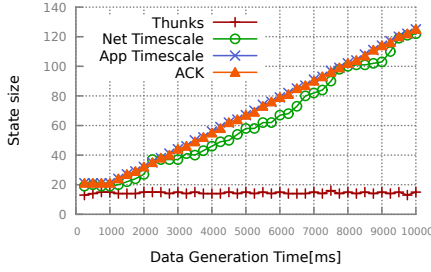
Figure 15: Forwarder state size.
