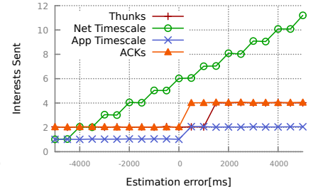
Figure 14: Number of Interests sent to retrieve a data chunk.
