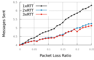
Figure 8: Handshake Overhead.
