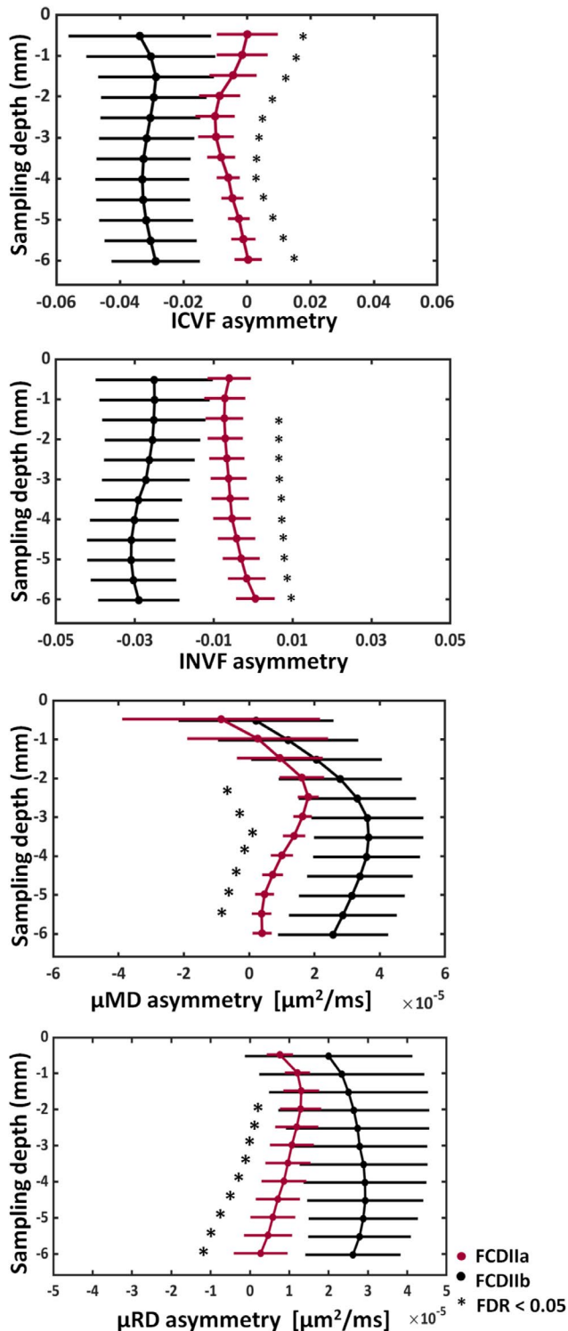
FIGURE 5 MRI profiling of the asymmetry for FCD IIa and IIb patients. Significant asymmetry differences at false discovery rate (FDR) < 0.05 (*), between histologically confirmed FCD IIb (black) and FCD IIa (red) patients were found on the ICVF, INVf, \mu MD, and \mu RD. The asymmetry was estimated by computing the difference vertex-wise between the lesion and homotopic region values using the maps showing significant changes between the two regions. The sampling depth is reported as a distance from the pial surface (0 mm). ICVF, intracellular volume fraction; INVf, intra-neurite volume fraction; \mu MD, \mu mean diffusivity; \mu RD, \mu Radial diffusivity; \mu AD, \mu Axial diffusivity. Error bars correspond to standard deviations computed over the cohort of patients
