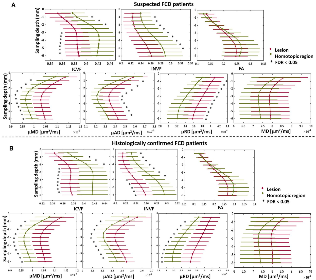
FIGURE 4 MRI profiling of FCD lesions and homotopic regions. A, MRI profiling of FCD lesions (red) and homotopic regions (green) for the new diffusion maps showing significant profile changes at false discovery rate (FDR) < 0.05 (*), and for MD, FA maps not providing significant differences for the whole patient cohort. The sampling depth is reported as a distance from the pial surface (0 mm). B, MRI profiling of FCD lesions (red) and homotopic (green) regions on histologically confirmed patients showing significant (false discovery rate [FDR] < 0.05) profile changes for all sampling depths on new diffusion maps in contrast to MD, FA maps. FA, fractional anisotropy; ICVF, intracellular volume fraction; INVf, intra-neurite volume fraction; MD, mean diffusivity; \mu\text{AD} , \mu axial diffusivity; \mu\text{MD} , \mu mean diffusivity; \mu\text{RD} , \mu radial diffusivity. Error bars correspond to standard deviations computed over the cohort of patients
