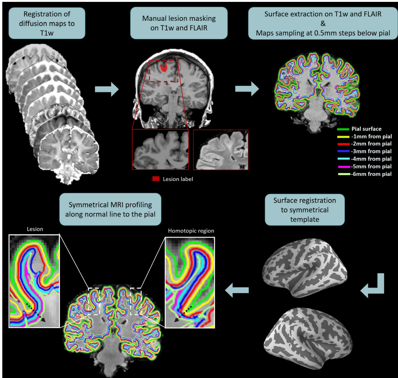
FIGURE 1 Maps sampling workflow. First, the new diffusion maps were coregistered to the T1-weighted (T1w) data. Manual lesion masking and surface extraction at increasing depths were performed on T1w and fluid-attenuated inversion recovery (FLAIR) images. The diffusion maps were projected onto the surfaces and sampled from the pial surface. Then, the surface sampling and the lesion masks were spatially registered to a symmetric template, allowing the symmetrical MRI profiling of the diffusion maps along the normal (black arrow) to the pial surface for the lesion and the homotopic region
