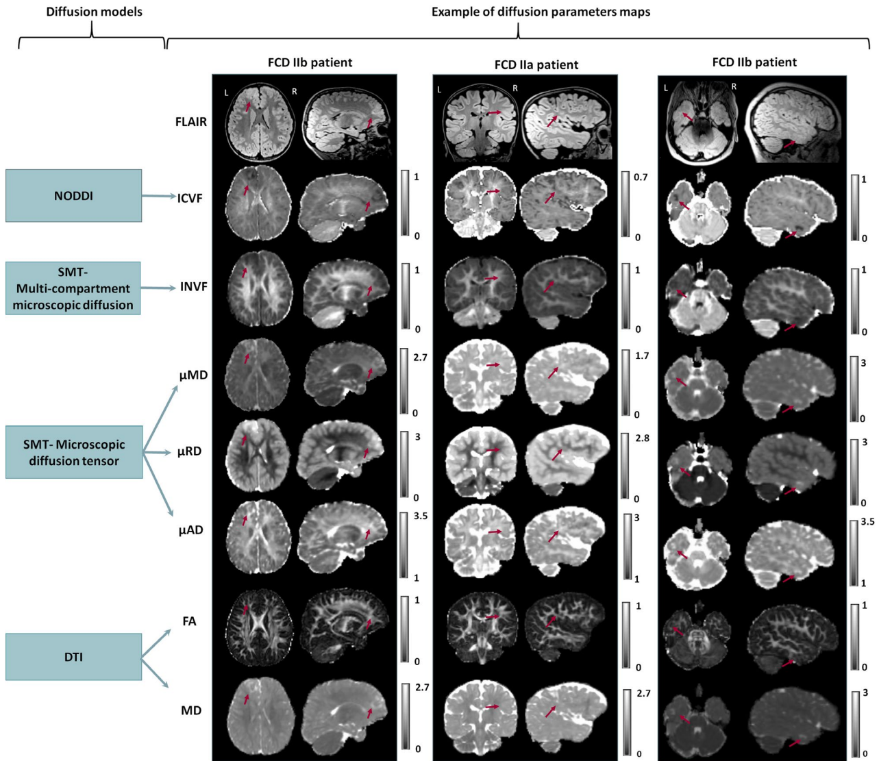
FIGURE 2 Diffusion models and examples of diffusion parameters maps were obtained in a clinical setting. Example of FLAIR, neurite orientation dispersion and density imaging (NODDI) intracellular volume fraction (ICVF), spherical mean technique (SMT) multi-compartment microscopic intra-neurite volume fraction (INVf), SMT microscopic mean diffusivity ( \mu MD), radial and axial diffusivities ( \mu RD and \mu AD), and standard DTI fractional anisotropy (FA) and mean diffusivity (MD) maps for three patients. (left) FCD IIB patient with very well-delineated lesion on all images except FA. (center) FCD IIA patient showing lesion is poorly delineated by FLAIR, FA, and MD but visible on ICVF and \mu RD maps. (right) FCD IIB patient showing the lesion is poorly delineated by FLAIR, FA, MD, but very well visible on ICVF, \mu MD, \mu RD, and \mu AD maps
