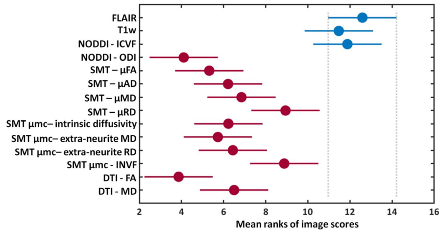
FIGURE 3 Multiple comparison test on the mean ranks of the image scores. The graph shows that the T1w and NODDI intracellular volume fraction (ICVF) have mean ranks not significantly different (blue) from FLAIR, whereas the other diffusion maps have mean ranks significantly different (red) from FLAIR images. Circles represent mean rank values, and error bars correspond to standard deviations. Extra-neurite MD, extra-neurite microscopic mean diffusivity; extra-neurite RD, extra-neurite microscopic radial diffusivity; INVf, intra-neurite volume fraction; ODI, orientation dispersion index; \mu AD, microscopic axial diffusivity; \mu FA, microscopic fractional anisotropy; \mu MD, microscopic mean diffusivity; \mu RD, microscopic radial diffusivity
