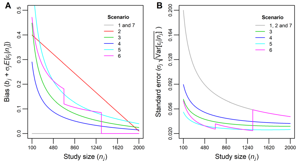
FIGURE 3 Illustration of the relationship between bias and n_j (panel A), and between standard error and n_j (panel B), induced by different models of small-study effects
