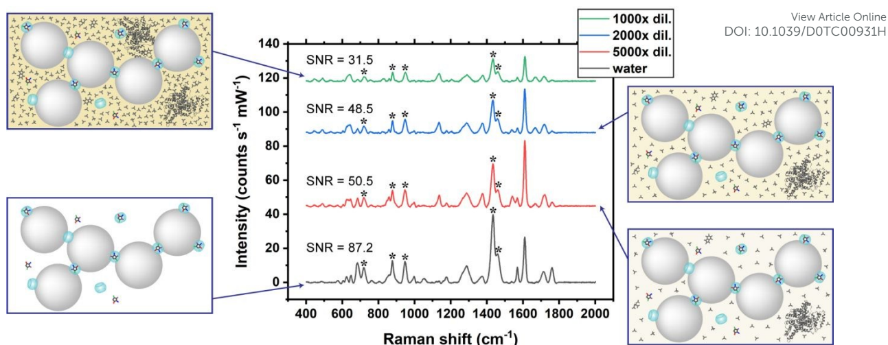
Figure 5. SERS spectra of 0.60 \mu\text{g/ml} CRN in water and SU after subsequent dilutions, showing the matrix effect on the SERS signals of CRN. The CRN signals (marked by asterisks) in water are gradually recovered and the SNR is higher as the concentration of SU is lowered.
