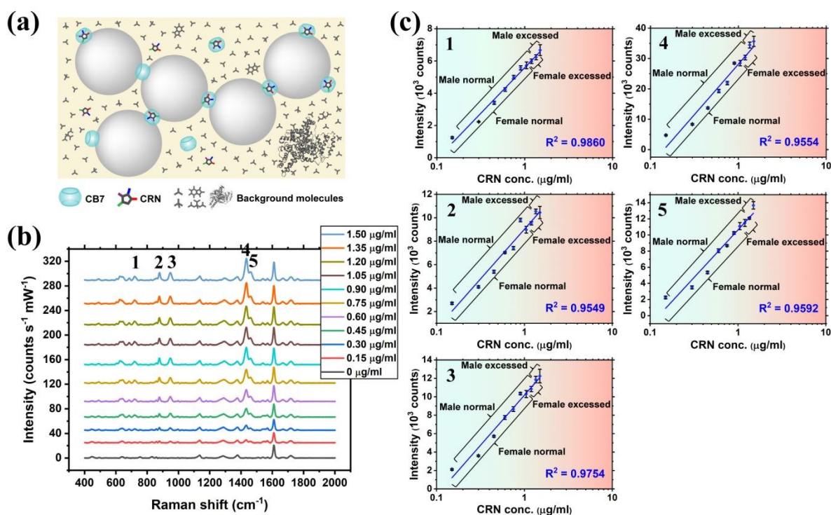
Figure 4. (a) Schematic illustration of the precise plasmonic hotspots within dynamic aggregates of Au NPs formed by 10 \mu\text{M} CB7 for CRN detection in SU after 2000x dilution with water (not to scale). (b) SERS spectra of CRN in SU with concentrations from 0 to 1.50 \mu\text{g/ml} (13.3 \mu\text{M} ) with aggregation of Au NPs triggered by 10 \mu\text{M} CB7. Spectra were baseline corrected and offset for clarity. (c) Corresponding plots of SERS intensity of the five characteristic CRN peaks in (b) against CRN concentration. Logarithmic fittings were performed to reveal correlation between SERS intensity and CRN concentration. (Note: 1 \mu\text{g/ml} in measurement samples corresponds to 2000 \mu\text{g/ml} of the actual CRN concentration in undiluted patient samples.)
