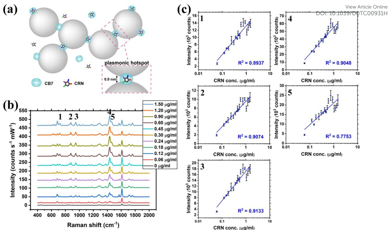
Figure 3. (a) Schematic illustration of the precise plasmonic hotspots within dynamic aggregates of Au NPs formed by 10 \mu\text{M} CB7 for CRN detection in water (not to scale). (b) SERS spectra of CRN in water with concentrations from 0 to 1.50 \mu\text{g/ml} (13.3 \mu\text{M} ) with aggregation of Au NPs triggered by 10 \mu\text{M} CB7 (See Figure S9 for all concentrations). Spectra were baseline corrected and offset for clarity. (c) Corresponding plots of SERS intensity of the five characteristic CRN peaks in (b) against CRN concentration. Logarithmic fittings were performed to reveal correlation between SERS intensity and CRN concentration.
