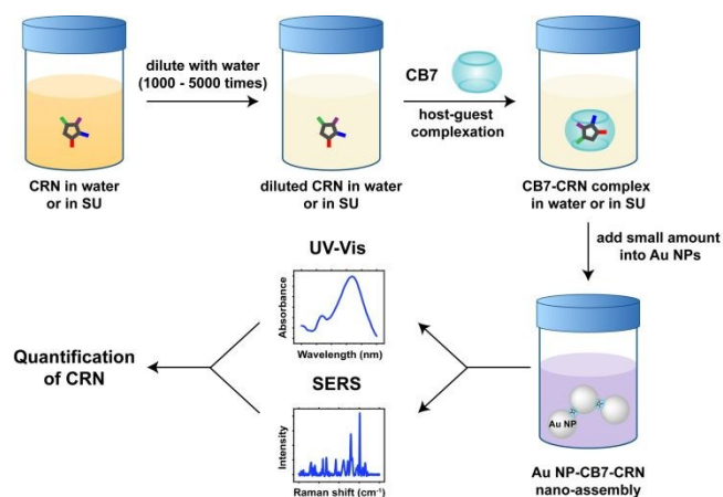
Figure 1. Schematic illustration of our dual UV-Vis and SERS detection scheme triggered by the formation of host-guest complexes between CB7 and CRN in highly diluted SU and the self-assembly of Au NPs mediated by portal binding of CB7 and electrostatic interactions with CRN.
