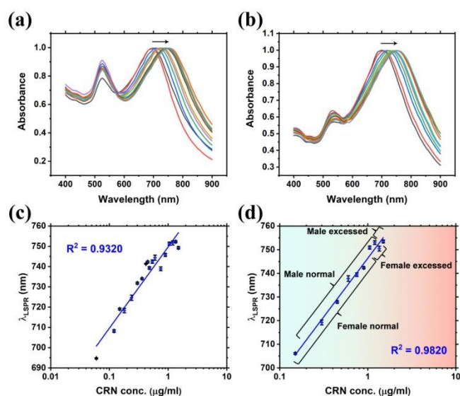
Figure 2. (a-b) UV-Vis spectra of CRN in (a) water (See Figure S5 for all concentrations) and (b) SU after 2000x dilution with concentrations from 0 to 1.50 \mu\text{g/ml} (13.3 \mu\text{M} ) with aggregation of Au NPs triggered by 10 \mu\text{M} CB7, with arrows indicating the shifting of the LSPR peaks. (c-d) Corresponding plots of \lambda_{\text{LSPR}} in (a-b) against CRN concentration respectively. Logarithmic fittings were performed to reveal correlation between \lambda_{\text{LSPR}} and CRN concentrations. (Note: 1 \mu\text{g/ml} in measurement samples corresponds to 2000 \mu\text{g/ml} of the actual CRN concentration in undiluted patient samples.)
