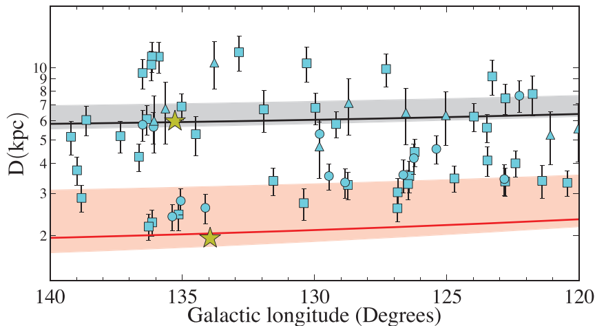
Figure 11. The spatial distribution of our CBe stars on the Galactic plane is shown. Different symbols are used for the luminosity class: dwarf (squares), circles (subgiants) and triangles (giants). The spiral arms are plotted following the prescriptions given in Vallée (2008) – solid red curve for the Perseus Arm, black solid curve for the Outer Arm. Instead, the two bands of width 1.4 kpc (Russeil et al. 2007) represent the range of distances that are covered by the two spiral arms in Russeil et al. (2007). The Perseus Arm is in pink, the Outer Arm is in grey. The two yellow stars mark the trigonometric parallaxes of masers as specified by Reid et al. (2009), which are sitting on the near edge of the spiral arms where the star formation is active.
