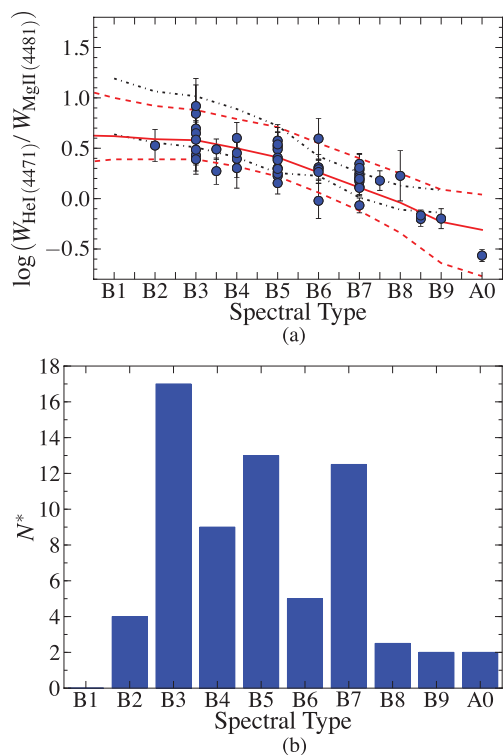
Figure 4. (a) Correlation between spectral type and the logarithm of the equivalent width ratio, W(\text{He I } \lambda 4471)/W(\text{Mg II } \lambda 4481) . Our sample is compared to an interpolation of the high-resolution data from Chauville et al. (2001): the black dotted curves mark the 1\sigma confidence limits. The dashed red curves, instead, represent the 1\sigma confidence limits obtained from repeated measures of equivalent width ratios from appropriately chosen model atmospheres, with random noise added that matches S/N = 40 . The blue circles are the values obtained for our sample. (b) The histogram of spectral subtypes in the CBE sample.
