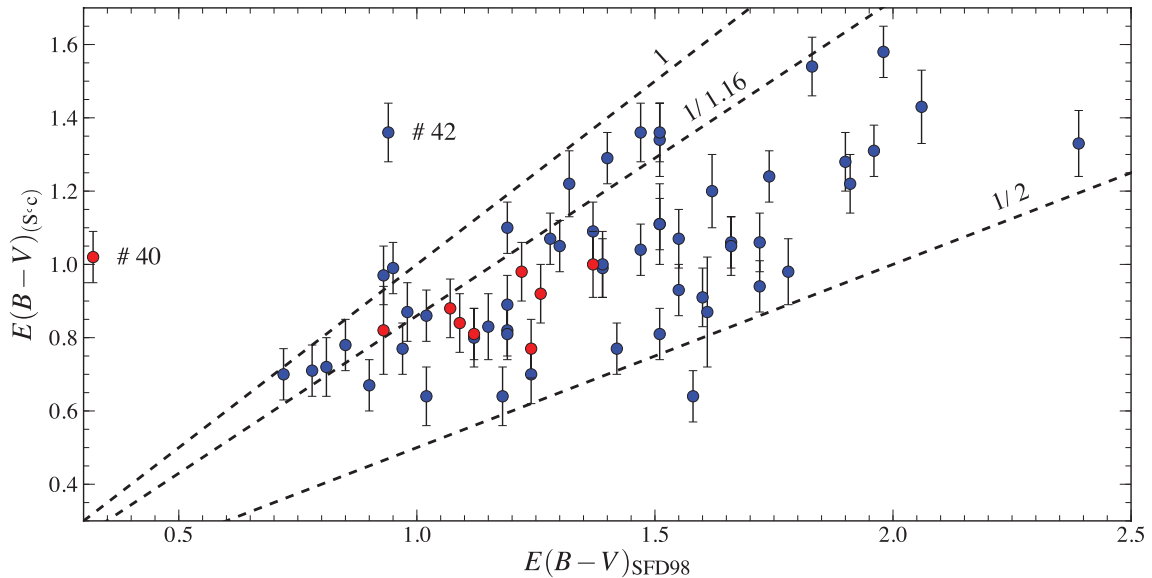
Figure 13. The corrected colour excesses for the CBe star sample is plotted against the corresponding integrated Galactic colour excesses from SFD98, for each sightline. The red symbols are used for the stars with a measured distance larger than 8 kpc, well beyond the expected location of the Outer Arm. The three dashed black lines are linear relations of the form E(B - V)_{(S,C)} = mE(B - V)_{SFD98} , where m = 1, 1/1.16, 1/2 , respectively.
