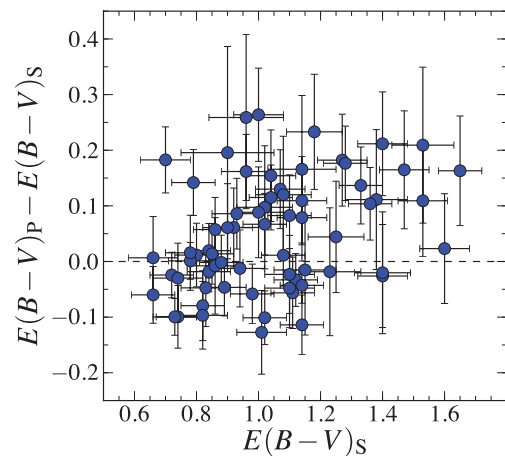
Figure 7. The difference between the two colour excess measurements, E(B - V)_P - E(B - V)_S is plotted as a function of the spectroscopic colour excess, E(B - V)_S . The data points are scattered with a bias to positive values, as expected, due to the reddening effect associated with the circumstellar disc emission present in these stars.
