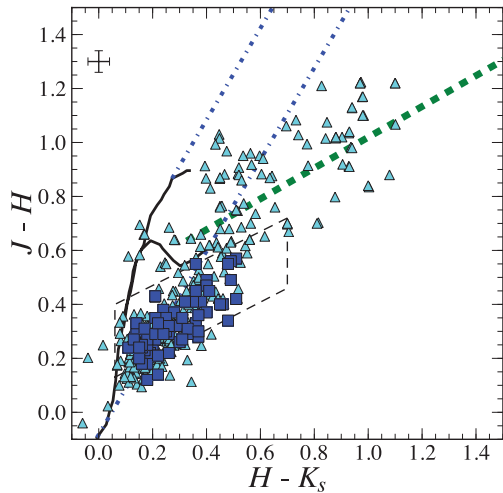
Figure 3. 2MASS NIR colour-colour diagram of our sample. The colour symbols are the same as in Fig. 1. The solid line follows the dwarf and giant unreddened sequences (Bessell & Brett 1988). The blue dot-dashed lines are the reddening vectors from Rieke & Lebofsky (1985). The box drawn is due to Corradi et al. (2008) and roughly delineates the region CBe stars with A_V \sim 4 would occupy, while the green dashed line is the CTTS locus (Meyer, Calvet & Hillenbrand 1997). All the plotted curves are converted to the 2MASS system, adopting relationships defined in Carpenter (2001). Typical error bars are in the upper-left corner of the diagram.
