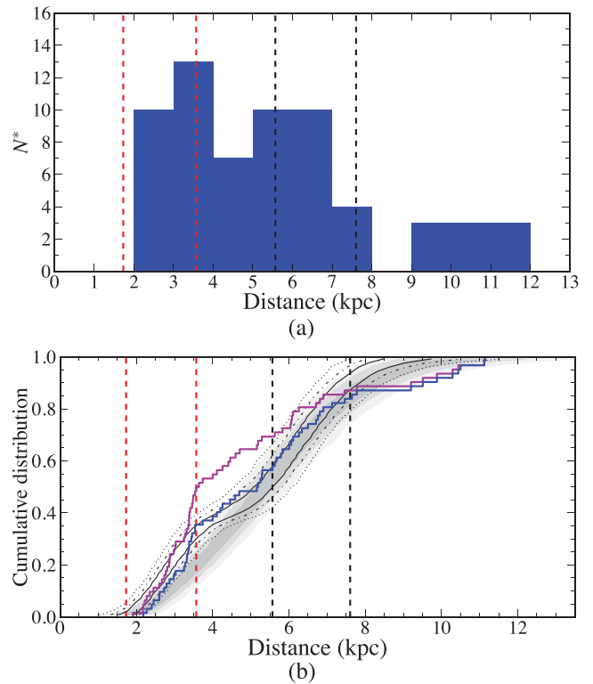
Figure 12. (a) Histogram distribution of stars with luminosity class being assigned according to Table 6. The vertical dashed lines define the distance ranges thought to be occupied by the spiral arms: red is used for the Perseus Arm, black for the Outer Arm. (b) The cumulative distribution of CBe stars is plotted against the distances derived from spectroscopic parallax. The blue curve expresses the distribution of stars that takes note of the preferred luminosity class assignment in Table 6. The dark magenta curve is the result obtained if all the CBe stars are assumed to be class V. The grey-scale contours represent the 1\sigma , 2\sigma and 3\sigma confidence limits that result from the MC simulations of a smooth distribution of stars. Similarly, the black curves are for the boundaries defined by the family of CDCs, which are derived from the MC simulations of stars within the spiral arms. The vertical dashed lines define the range of distances associated with the spiral arms, as in panel (a).
