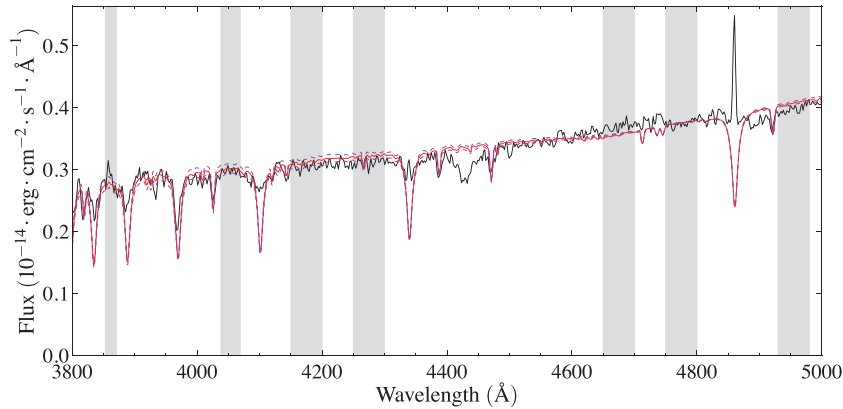
Figure 6. Example of a reddening measurement based on a blue spectrum. The INT spectrum of object #16 (black line) is shown along with the model atmosphere for T_{\text{eff}} = 17000\text{K} , reddened according to the best-fitting colour excess ( E(B - V)_S = 1.27 \pm 0.04 ). The reddened model is drawn in red, with its 1\sigma error bounds shown as purple dashed lines. The shaded vertical strips pick out the continuum intervals used in the fitting procedure. The normalization applied in this instance is at \lambda 4775 \text{ \AA} . Note that the poor agreement between the template Balmer line profiles and those of the star is due to infilling line emission.
