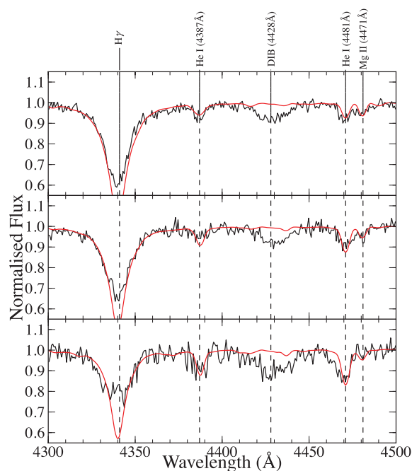
Figure 5. Examples of spectral type assignments based on three spectra with different S/N ratio. From top to bottom, #41 (B7, S/N = 64 ), #65 (B5, S/N = 48 ), #50 (B3, S/N = 34 ). The observed spectra are in black while the preferred Munari et al. (2005) models are in red. The models have been rebinned to match that of the observations.
