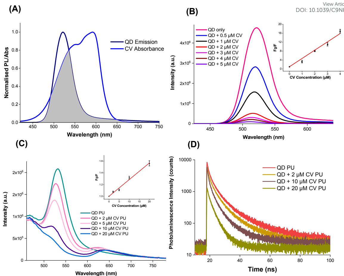
Figure 3. (A) Spectral overlap of QD emission and crystal violet absorbance. PL excitation at 400 nm. (B) Emission of QD with increasing CV concentration in solution at 400 nm excitation. Inset: S-V relationship of QD quenching vs. CV concentration in solution at 500 nm. (C) Emission of QD alone or in combination with increasing concentrations of CV into polyurethane (excitation at 400 nm). Inset: Stern-Volmer plot of QD fluorescence quenching ratio vs. CV concentration in polyurethane at 500 nm. (D) Time-resolved emission of QD alone or in combination with increasing concentrations of CV in polyurethane.
